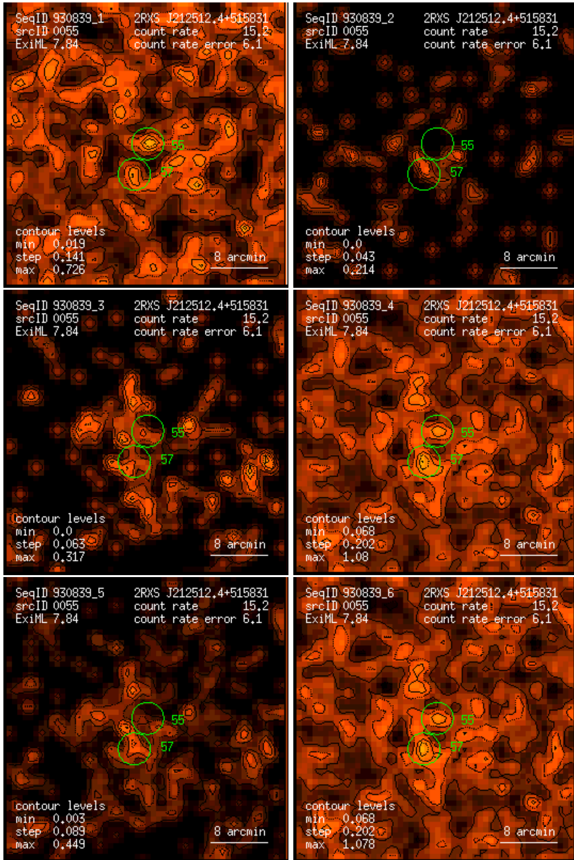
Figure 55: RASS 930839: detection 0055: band rate images, Gaussian filter: (1) PSPC channels 11 – 41, (2) 52 – 90, (3) 91 – 201, (4) 11 – 235, (5) 52 – 201, (6) 11 – 201. Broad band rates in counts/ks. Band rate contour levels in counts/ks/arcmin 2 .
