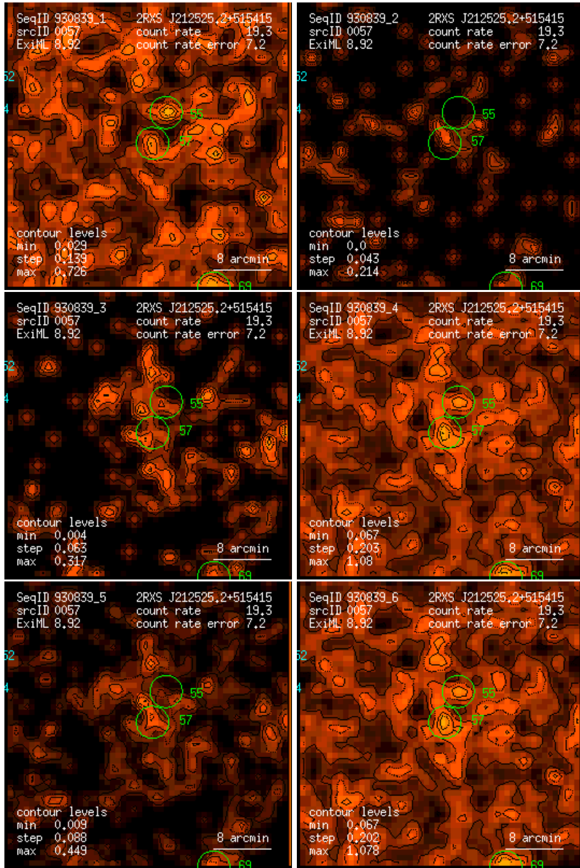
Figure 57: RASS 930839: detection 0057: band rate images, Gaussian filter: (1) PSPC channels 11 – 41, (2) 52 – 90, (3) 91 – 201, (4) 11 – 235, (5) 52 – 201, (6) 11 – 201. Broad band rates in counts/ks. Band rate contour levels in counts/ks/arcmin 2 .
