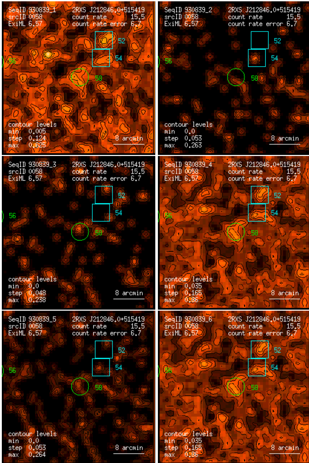
Figure 58: RASS 930839: detection 0058: band rate images, Gaussian filter: (1) PSPC channels 11 – 41, (2) 52 – 90, (3) 91 – 201, (4) 11 – 235, (5) 52 – 201, (6) 11 – 201. Broad band rates in counts/ks. Band rate contour levels in counts/ks/arcmin 2 .
