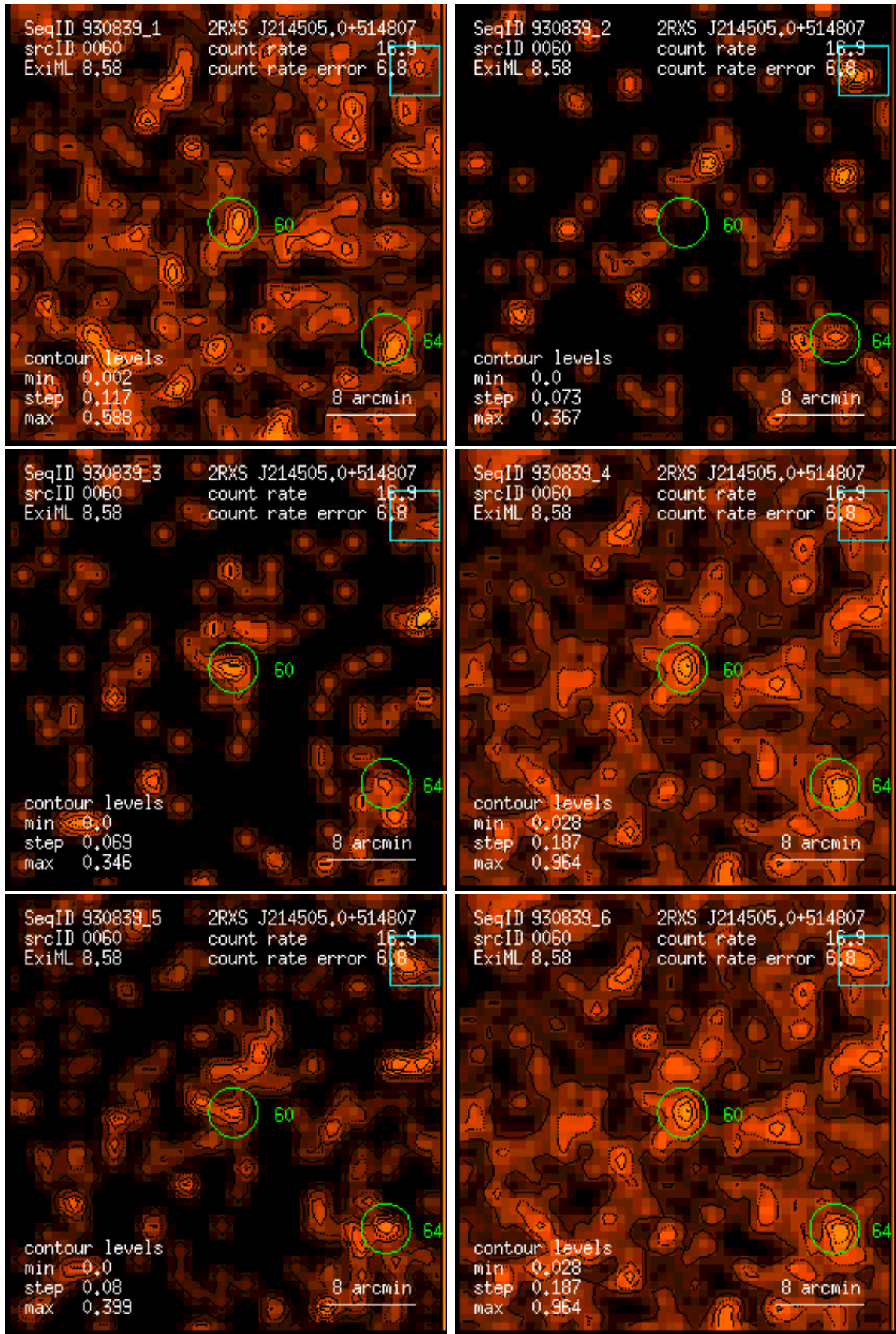
Figure 60: RASS 930839: detection 0060: band rate images, Gaussian filter: (1) PSPC channels 11 – 41, (2) 52 – 90, (3) 91 – 201, (4) 11 – 235, (5) 52 – 201, (6) 11 – 201. Broad band rates in counts/ks. Band rate contour levels in counts/ks/arcmin 2 .
