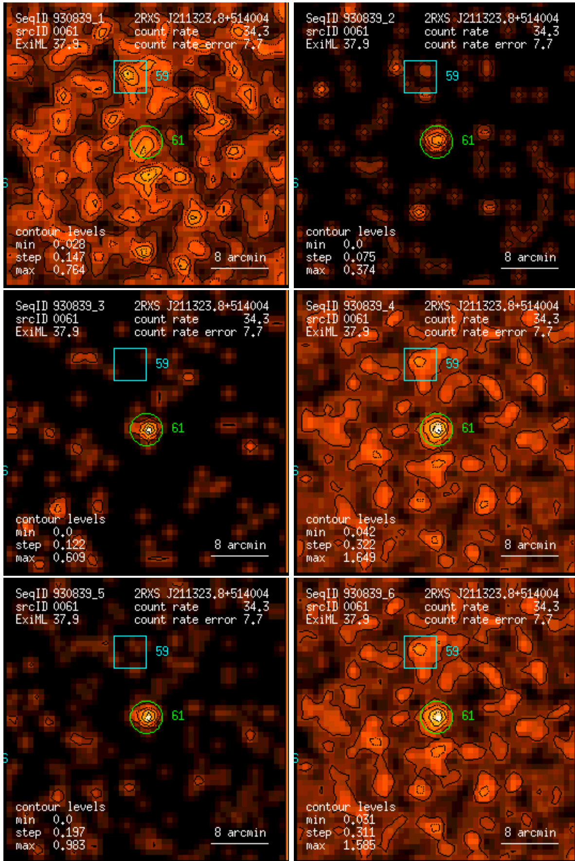
Figure 61: RASS 930839: detection 0061: band rate images, Gaussian filter: (1) PSPC channels 11 – 41, (2) 52 – 90, (3) 91 – 201, (4) 11 – 235, (5) 52 – 201, (6) 11 – 201. Broad band rates in counts/ks. Band rate contour levels in counts/ks/arcmin 2 .
