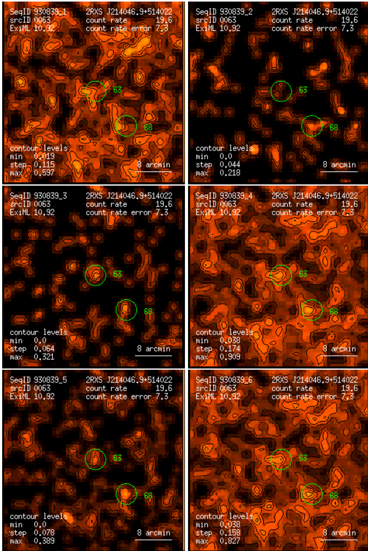
Figure 63: RASS 930839: detection 0063: band rate images, Gaussian filter: (1) PSPC channels 11 – 41, (2) 52 – 90, (3) 91 – 201, (4) 11 – 235, (5) 52 – 201, (6) 11 – 201. Broad band rates in counts/ks. Band rate contour levels in counts/ks/arcmin 2 .
