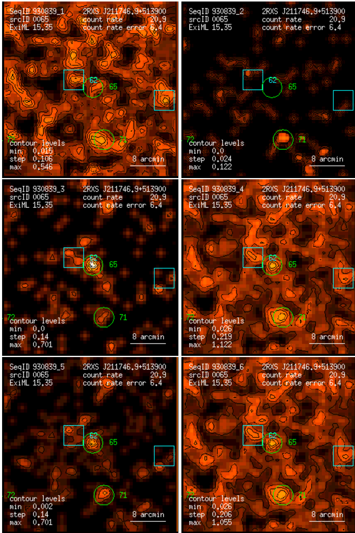
Figure 65: RASS 930839: detection 0065: band rate images, Gaussian filter: (1) PSPC channels 11 – 41, (2) 52 – 90, (3) 91 – 201, (4) 11 – 235, (5) 52 – 201, (6) 11 – 201. Broad band rates in counts/ks. Band rate contour levels in counts/ks/arcmin 2 .
