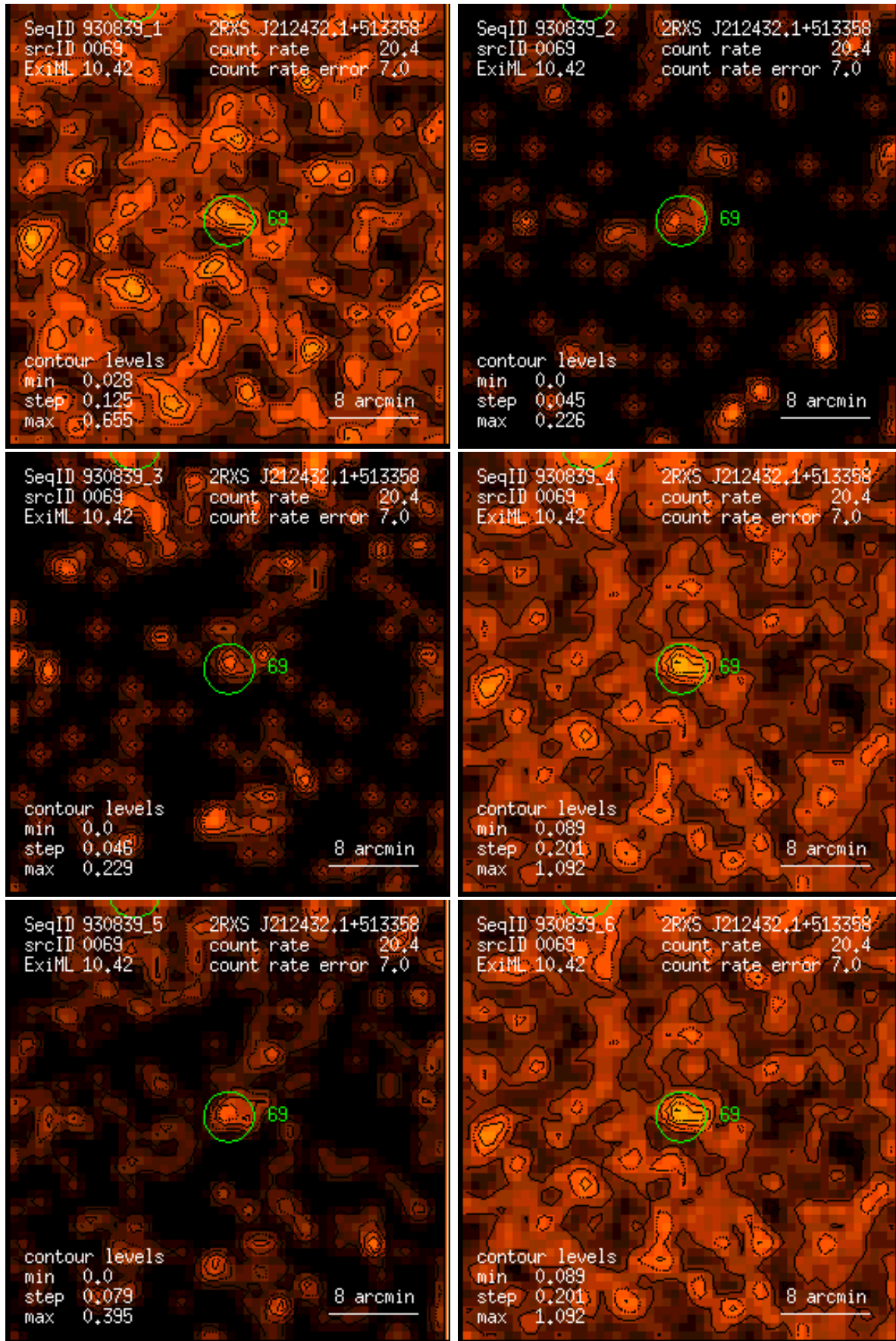
Figure 69: RASS 930839: detection 0069: band rate images, Gaussian filter: (1) PSPC channels 11 – 41, (2) 52 – 90, (3) 91 – 201, (4) 11 – 235, (5) 52 – 201, (6) 11 – 201. Broad band rates in counts/ks. Band rate contour levels in counts/ks/arcmin 2 .
