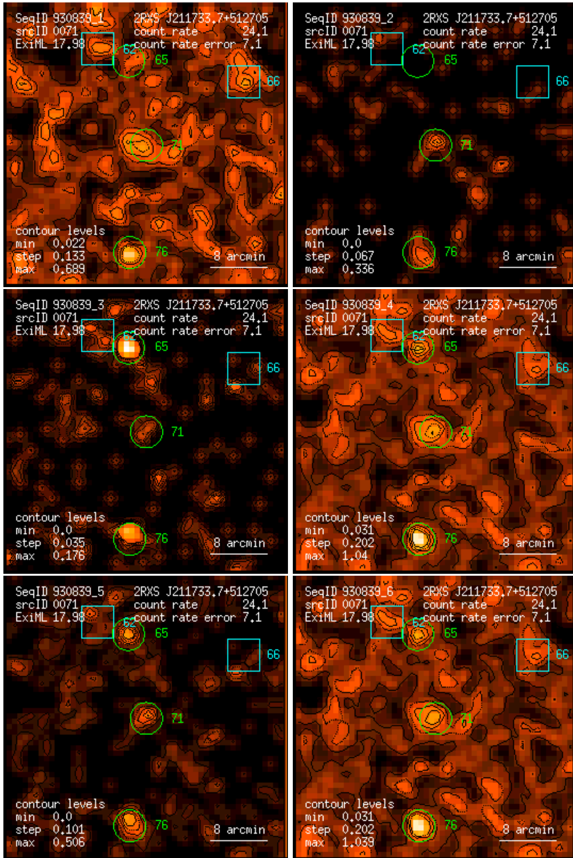
Figure 71: RASS 930839: detection 0071: band rate images, Gaussian filter: (1) PSPC channels 11 – 41, (2) 52 – 90, (3) 91 – 201, (4) 11 – 235, (5) 52 – 201, (6) 11 – 201. Broad band rates in counts/ks. Band rate contour levels in counts/ks/arcmin 2 .
