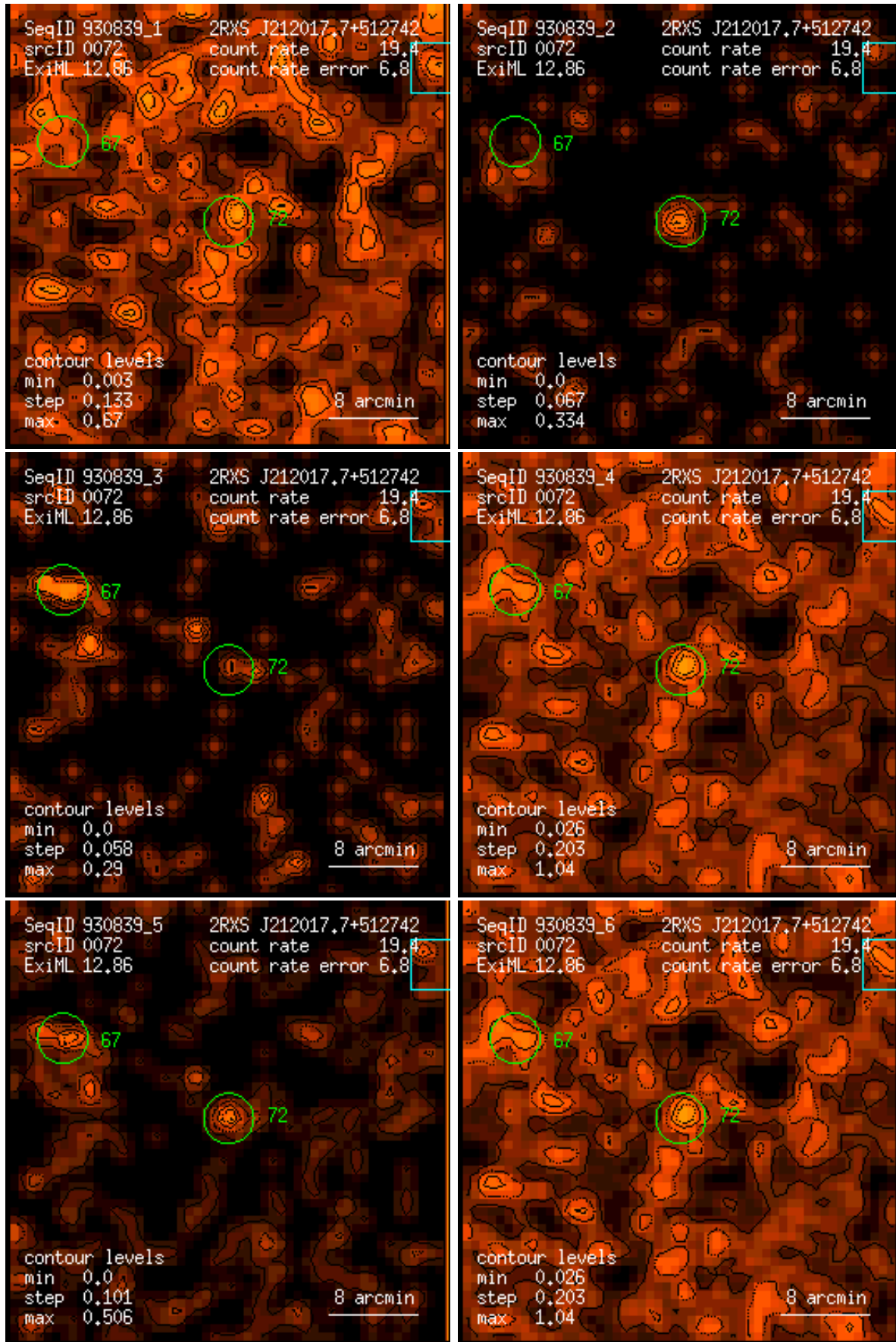
Figure 72: RASS 930839: detection 0072: band rate images, Gaussian filter: (1) PSPC channels 11 – 41, (2) 52 – 90, (3) 91 – 201, (4) 11 – 235, (5) 52 – 201, (6) 11 – 201. Broad band rates in counts/ks. Band rate contour levels in counts/ks/arcmin 2 .
