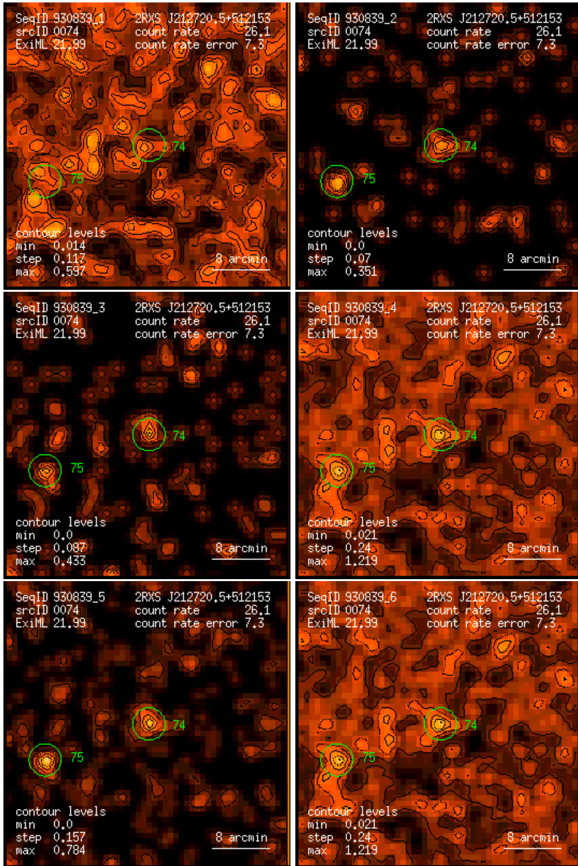
Figure 74: RASS 930839: detection 0074: band rate images, Gaussian filter: (1) PSPC channels 11 – 41, (2) 52 – 90, (3) 91 – 201, (4) 11 – 235, (5) 52 – 201, (6) 11 – 201. Broad band rates in counts/ks. Band rate contour levels in counts/ks/arcmin 2 .
