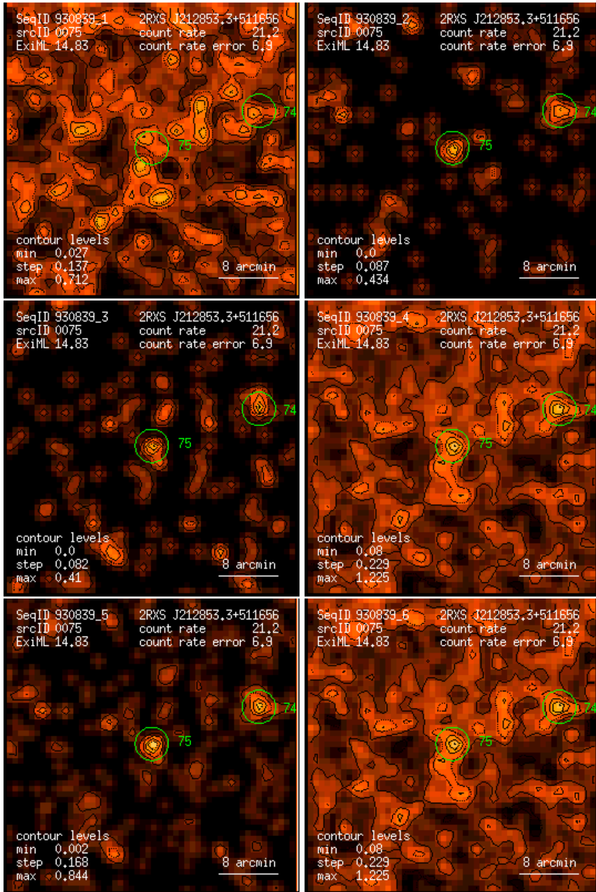
Figure 75: RASS 930839: detection 0075: band rate images, Gaussian filter: (1) PSPC channels 11 – 41, (2) 52 – 90, (3) 91 – 201, (4) 11 – 235, (5) 52 – 201, (6) 11 – 201. Broad band rates in counts/ks. Band rate contour levels in counts/ks/arcmin 2 .
