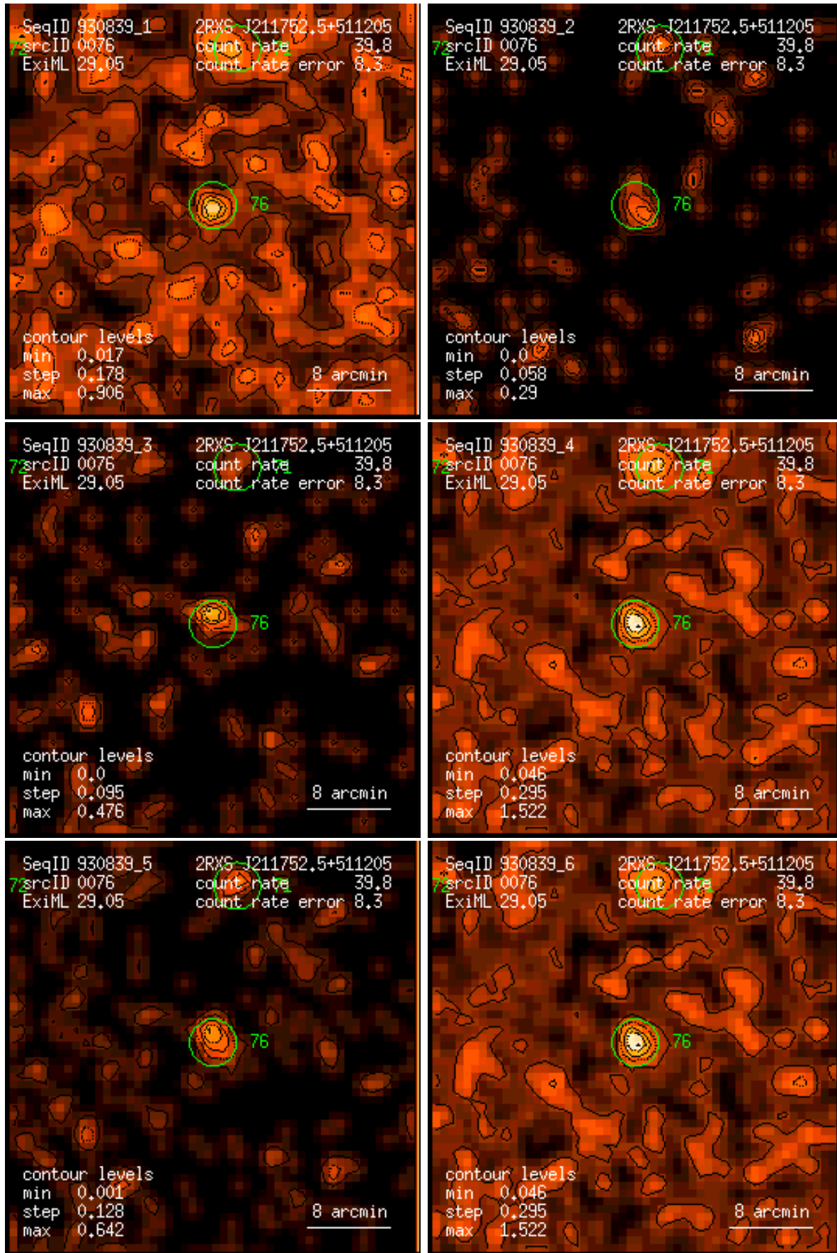
Figure 76: RASS 930839: detection 0076: band rate images, Gaussian filter: (1) PSPC channels 11 – 41, (2) 52 – 90, (3) 91 – 201, (4) 11 – 235, (5) 52 – 201, (6) 11 – 201. Broad band rates in counts/ks. Band rate contour levels in counts/ks/arcmin 2 .
