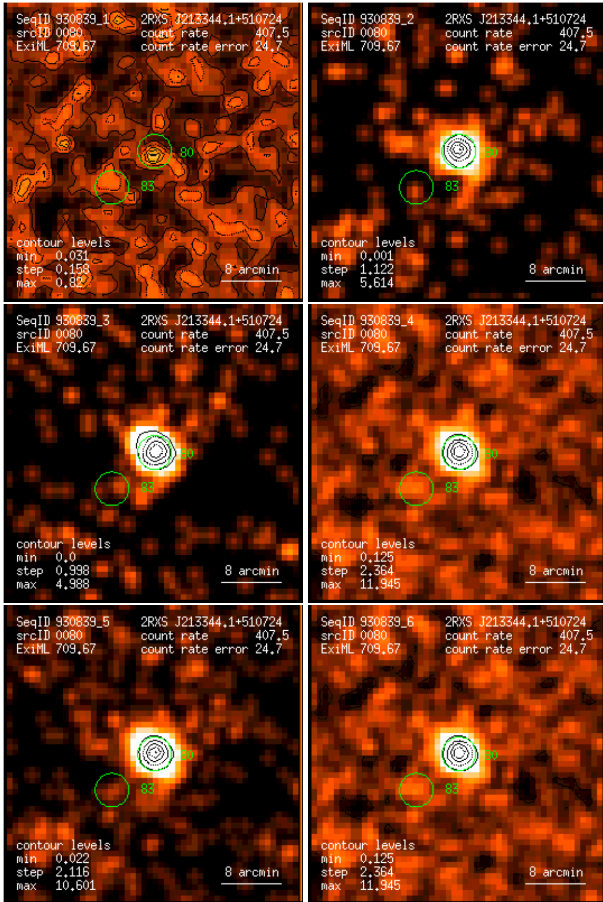
Figure 80: RASS 930839: detection 0080: band rate images, Gaussian filter: (1) PSPC channels 11 – 41, (2) 52 – 90, (3) 91 – 201, (4) 11 – 235, (5) 52 – 201, (6) 11 – 201. Broad band rates in counts/ks. Band rate contour levels in counts/ks/arcmin 2 .
