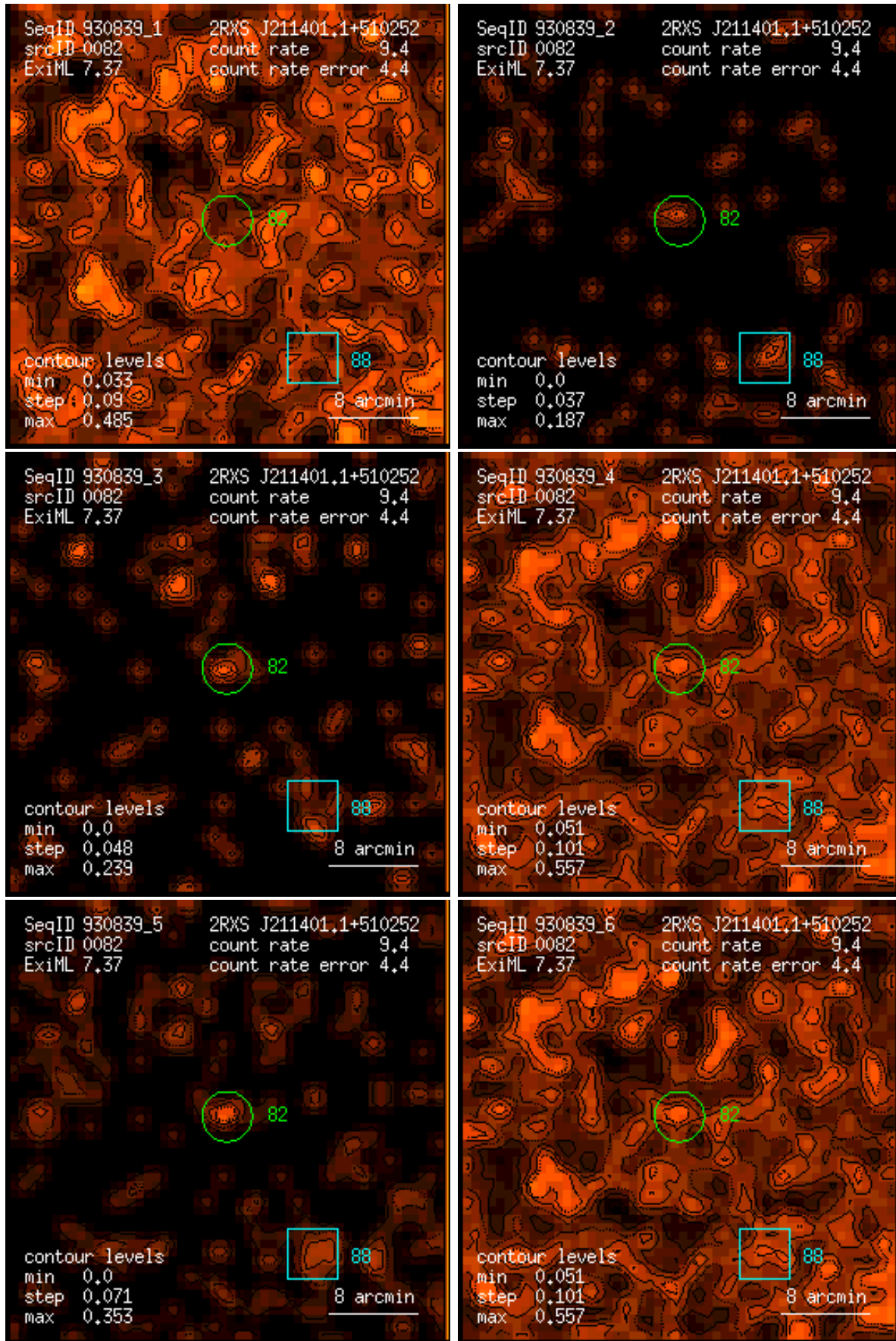
Figure 82: RASS 930839: detection 0082: band rate images, Gaussian filter: (1) PSPC channels 11 – 41, (2) 52 – 90, (3) 91 – 201, (4) 11 – 235, (5) 52 – 201, (6) 11 – 201. Broad band rates in counts/ks. Band rate contour levels in counts/ks/arcmin 2 .
