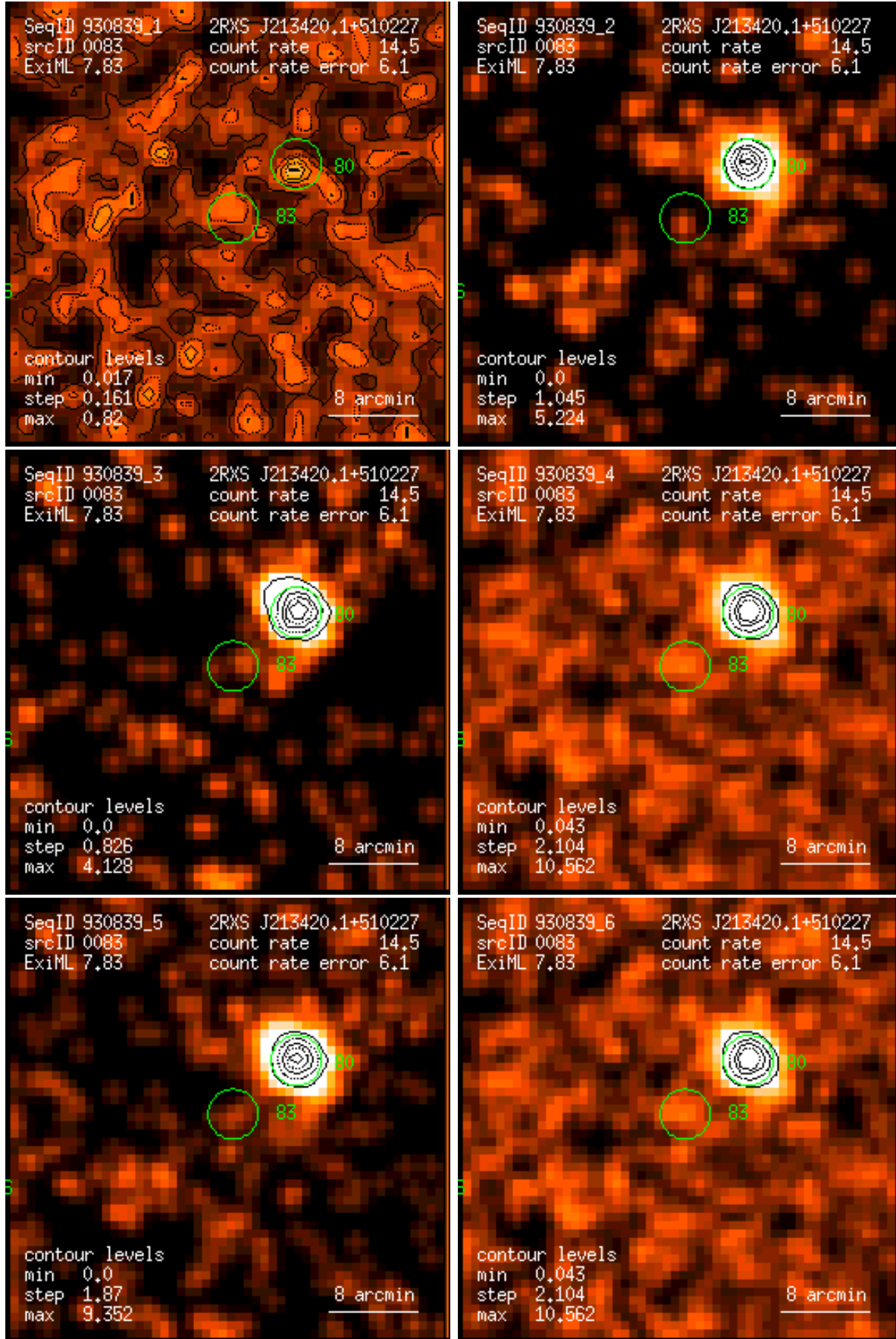
Figure 83: RASS 930839: detection 0083: band rate images, Gaussian filter: (1) PSPC channels 11 – 41, (2) 52 – 90, (3) 91 – 201, (4) 11 – 235, (5) 52 – 201, (6) 11 – 201. Broad band rates in counts/ks. Band rate contour levels in counts/ks/arcmin 2 .
