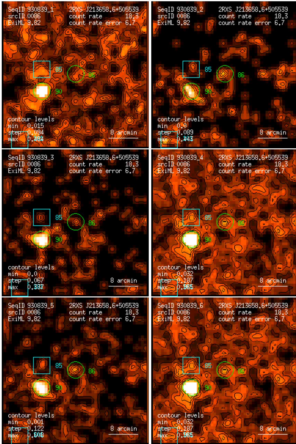
Figure 86: RASS 930839: detection 0086: band rate images, Gaussian filter: (1) PSPC channels 11 – 41, (2) 52 – 90, (3) 91 – 201, (4) 11 – 235, (5) 52 – 201, (6) 11 – 201. Broad band rates in counts/ks. Band rate contour levels in counts/ks/arcmin 2 .
