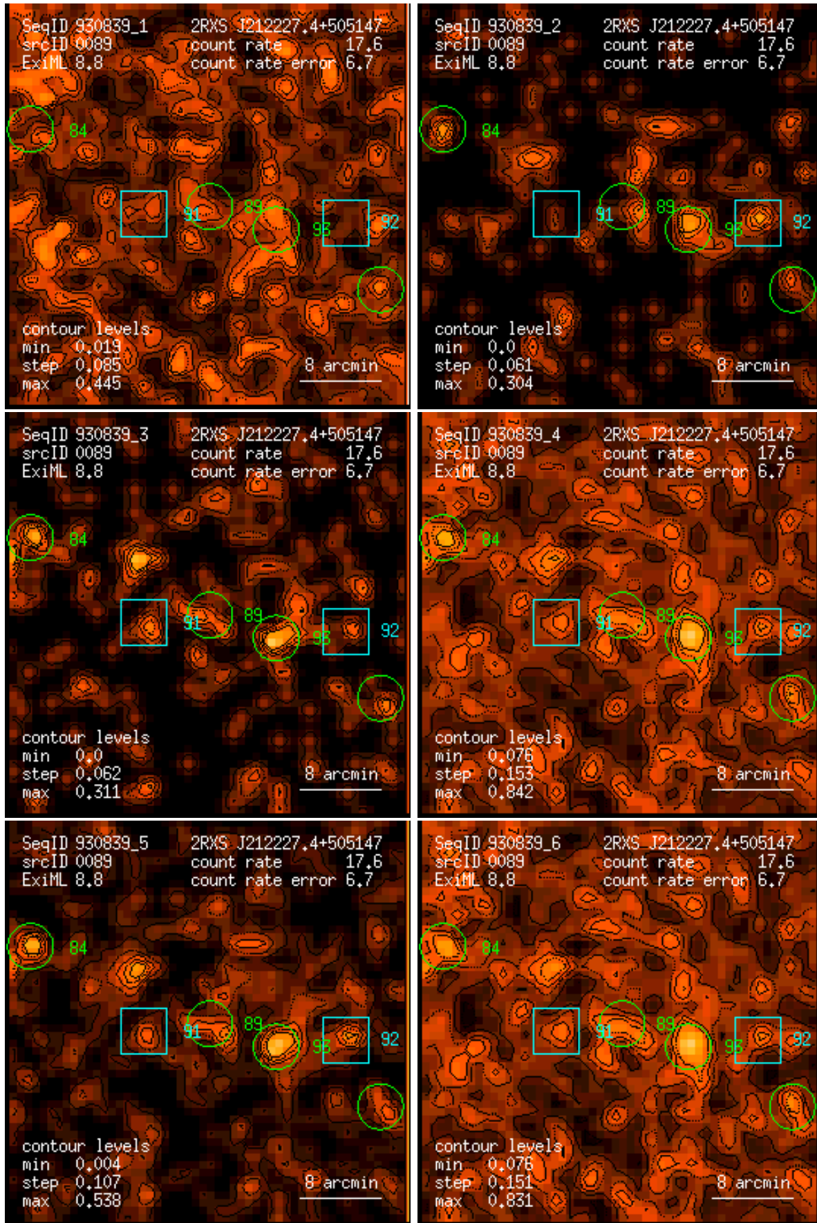
Figure 89: RASS 930839: detection 0089: band rate images, Gaussian filter: (1) PSPC channels 11 – 41, (2) 52 – 90, (3) 91 – 201, (4) 11 – 235, (5) 52 – 201, (6) 11 – 201. Broad band rates in counts/ks. Band rate contour levels in counts/ks/arcmin 2 .
