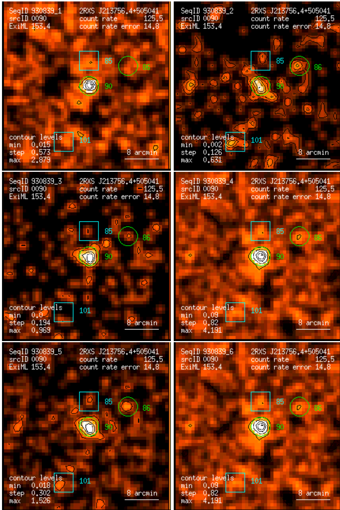
Figure 90: RASS 930839: detection 0090: band rate images, Gaussian filter: (1) PSPC channels 11 – 41, (2) 52 – 90, (3) 91 – 201, (4) 11 – 235, (5) 52 – 201, (6) 11 – 201. Broad band rates in counts/ks. Band rate contour levels in counts/ks/arcmin 2 .
