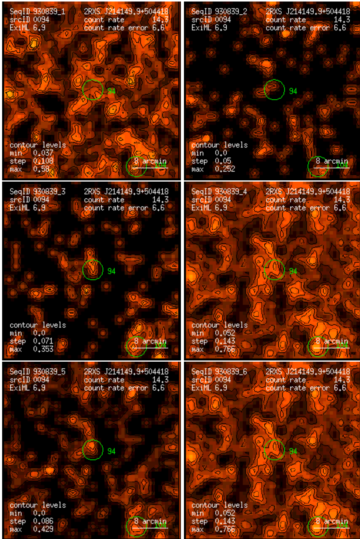
Figure 94: RASS 930839: detection 0094: band rate images, Gaussian filter: (1) PSPC channels 11 – 41, (2) 52 – 90, (3) 91 – 201, (4) 11 – 235, (5) 52 – 201, (6) 11 – 201. Broad band rates in counts/ks. Band rate contour levels in counts/ks/arcmin 2 .
