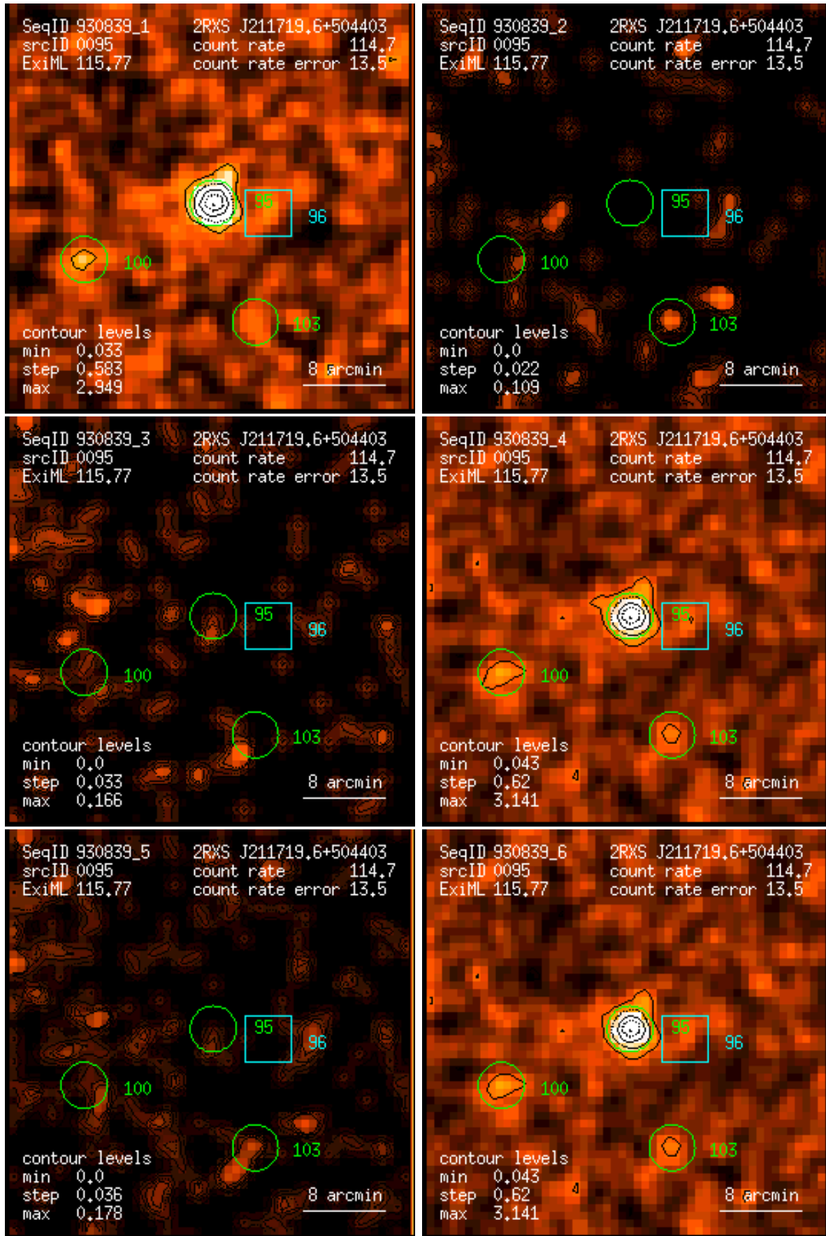
Figure 95: RASS 930839: detection 0095: band rate images, Gaussian filter: (1) PSPC channels 11 – 41, (2) 52 – 90, (3) 91 – 201, (4) 11 – 235, (5) 52 – 201, (6) 11 – 201. Broad band rates in counts/ks. Band rate contour levels in counts/ks/arcmin 2 .
