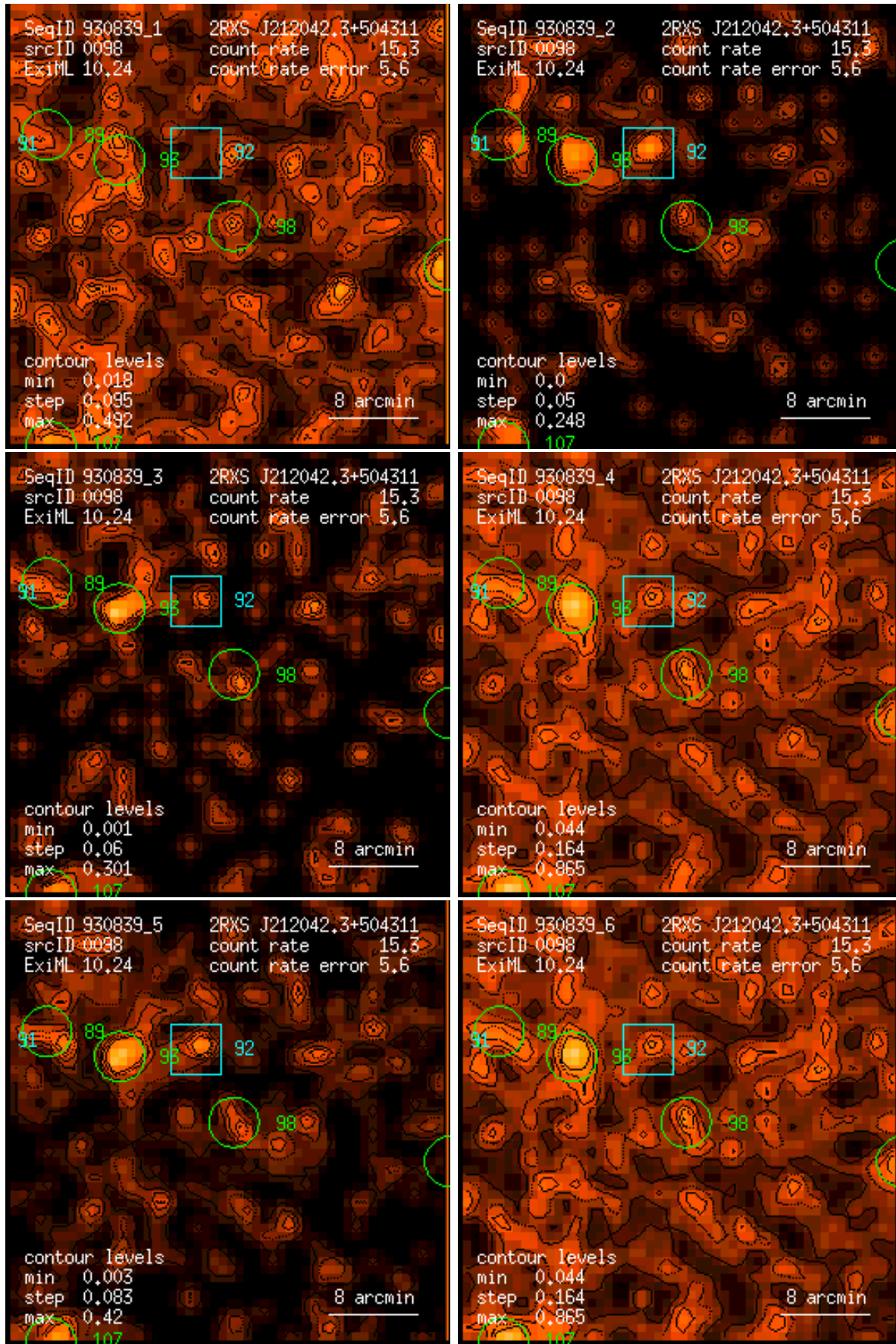
Figure 98: RASS 930839: detection 0098: band rate images, Gaussian filter: (1) PSPC channels 11 – 41, (2) 52 – 90, (3) 91 – 201, (4) 11 – 235, (5) 52 – 201, (6) 11 – 201. Broad band rates in counts/ks. Band rate contour levels in counts/ks/arcmin 2 .
