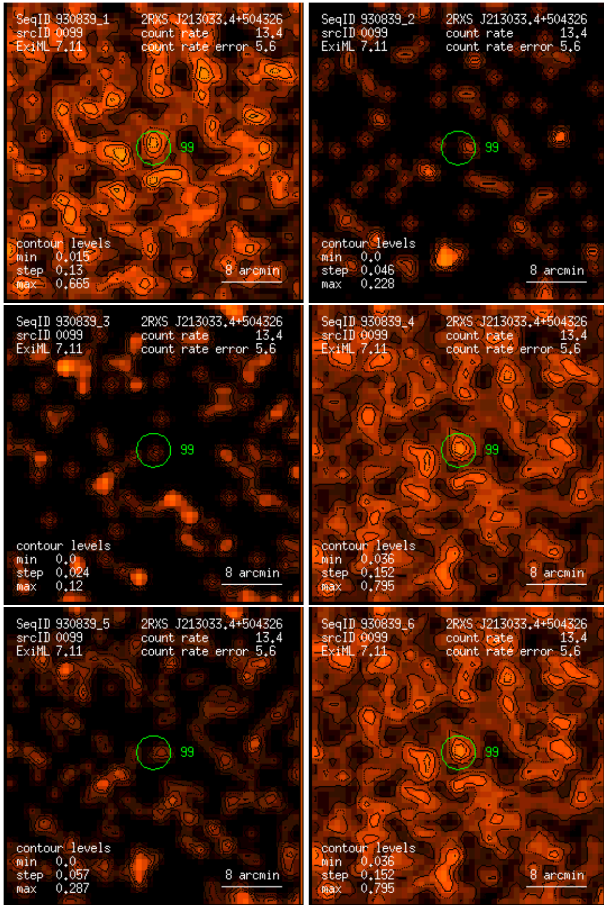
Figure 99: RASS 930839: detection 0099: band rate images, Gaussian filter: (1) PSPC channels 11 – 41, (2) 52 – 90, (3) 91 – 201, (4) 11 – 235, (5) 52 – 201, (6) 11 – 201. Broad band rates in counts/ks. Band rate contour levels in counts/ks/arcmin 2 .
