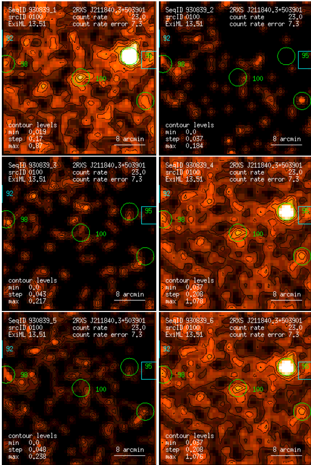
Figure 100: RASS 930839: detection 0100: band rate images, Gaussian filter: (1) PSPC channels 11 – 41, (2) 52 – 90, (3) 91 – 201, (4) 11 – 235, (5) 52 – 201, (6) 11 – 201. Broad band rates in counts/ks. Band rate contour levels in counts/ks/arcmin 2 .
