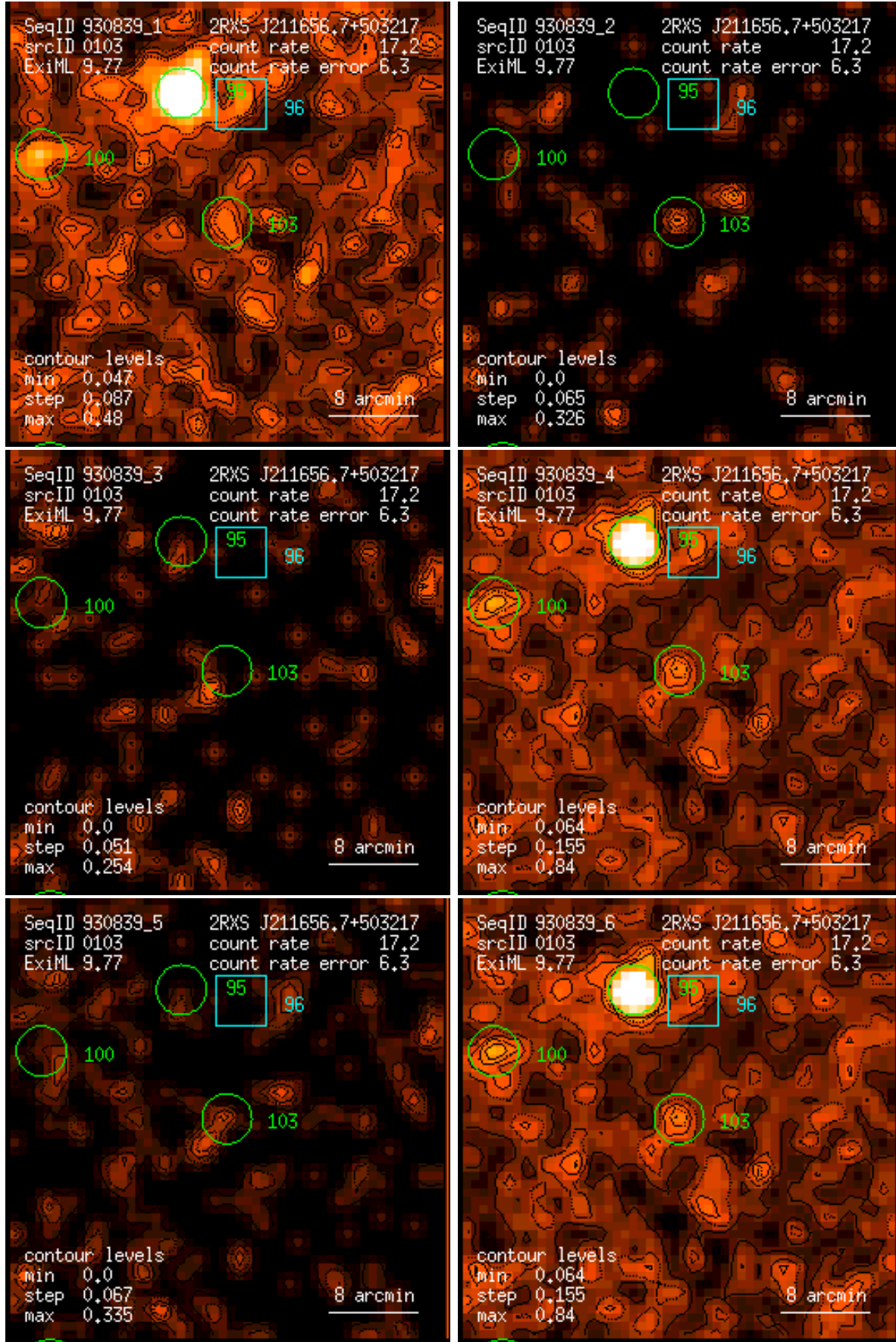
Figure 103: RASS 930839: detection 0103: band rate images, Gaussian filter: (1) PSPC channels 11 – 41, (2) 52 – 90, (3) 91 – 201, (4) 11 – 235, (5) 52 – 201, (6) 11 – 201. Broad band rates in counts/ks. Band rate contour levels in counts/ks/arcmin 2 .
