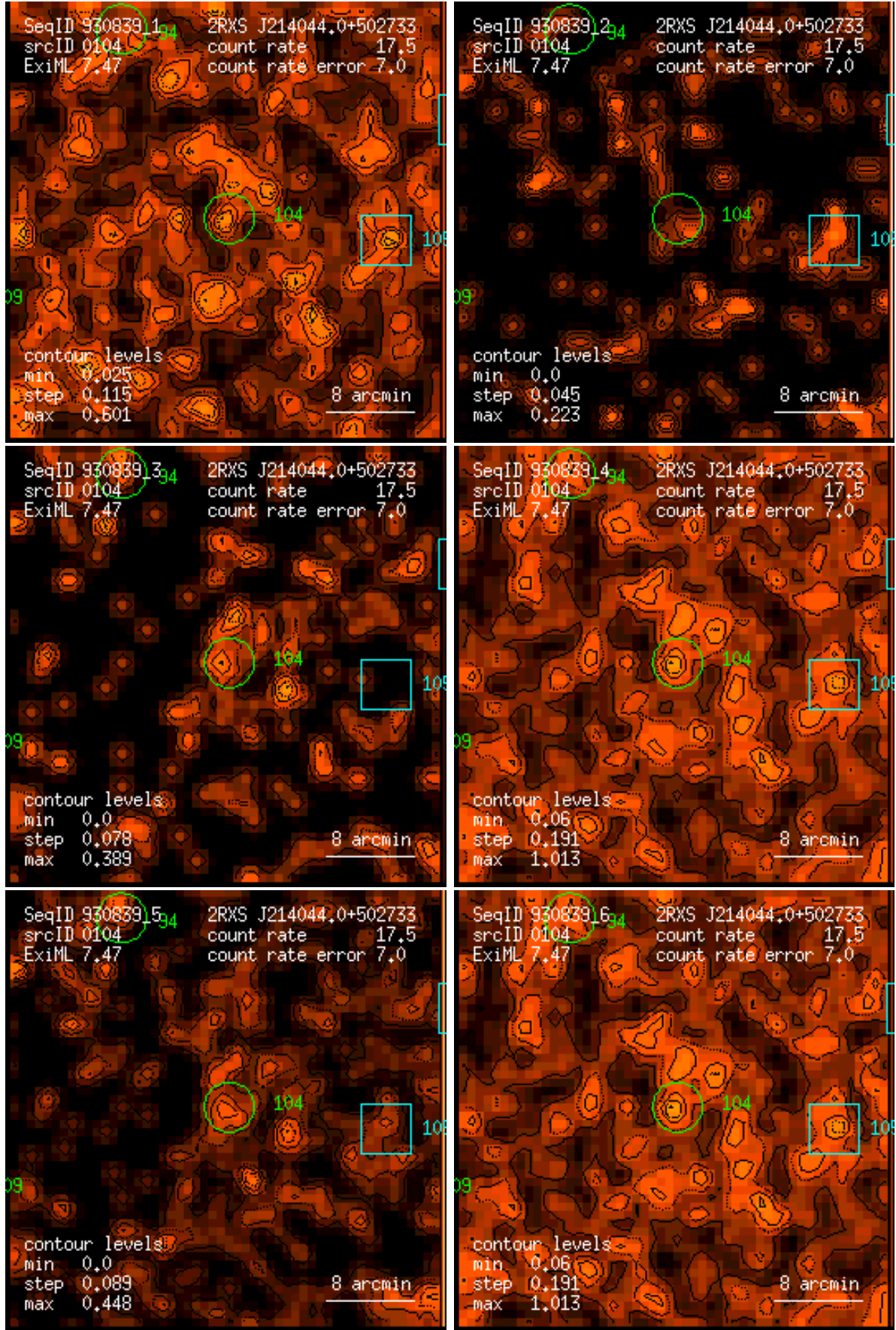
Figure 104: RASS 930839: detection 0104: band rate images, Gaussian filter: (1) PSPC channels 11 – 41, (2) 52 – 90, (3) 91 – 201, (4) 11 – 235, (5) 52 – 201, (6) 11 – 201. Broad band rates in counts/ks. Band rate contour levels in counts/ks/arcmin 2 .
