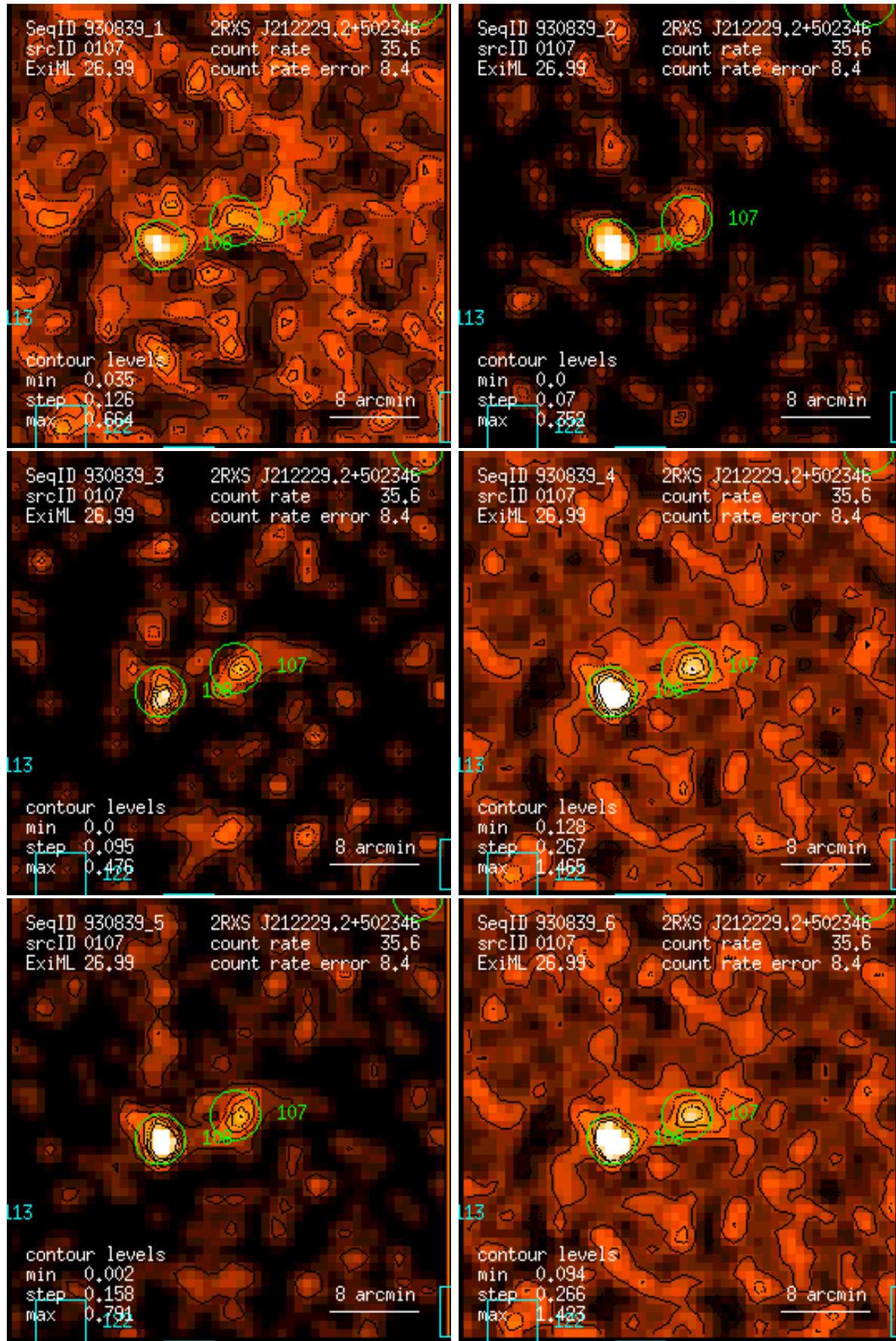
Figure 107: RASS 930839: detection 0107: band rate images, Gaussian filter: (1) PSPC channels 11 – 41, (2) 52 – 90, (3) 91 – 201, (4) 11 – 235, (5) 52 – 201, (6) 11 – 201. Broad band rates in counts/ks. Band rate contour levels in counts/ks/arcmin 2 .
