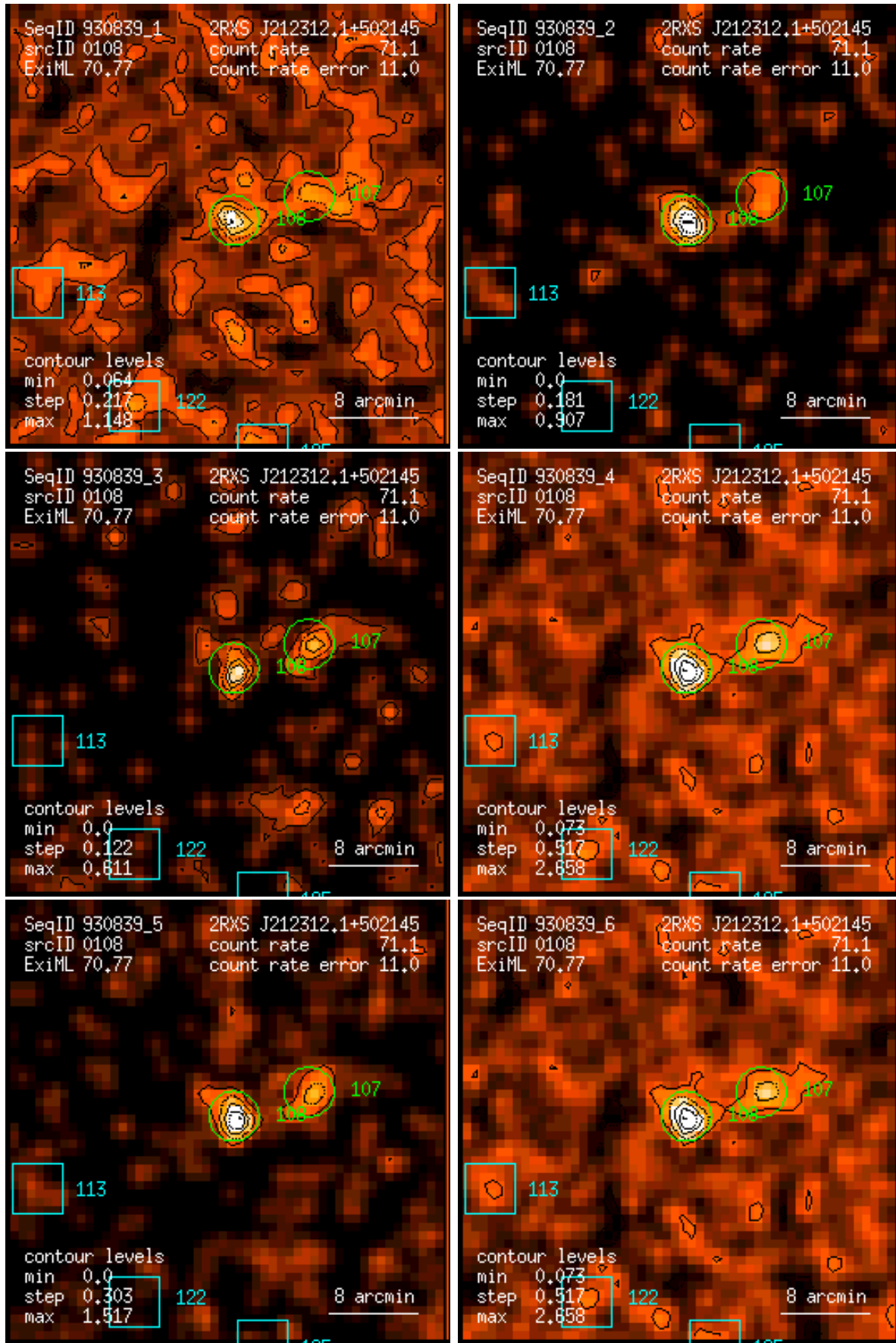
Figure 108: RASS 930839: detection 0108: band rate images, Gaussian filter: (1) PSPC channels 11 – 41, (2) 52 – 90, (3) 91 – 201, (4) 11 – 235, (5) 52 – 201, (6) 11 – 201. Broad band rates in counts/ks. Band rate contour levels in counts/ks/arcmin 2 .
