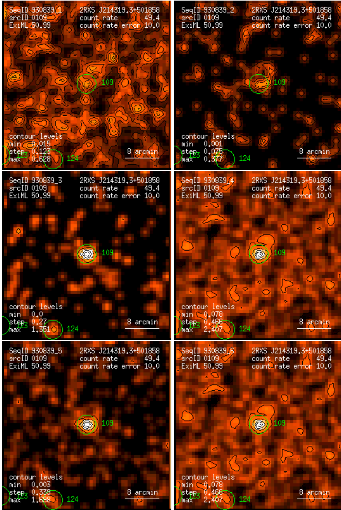
Figure 109: RASS 930839: detection 0109: band rate images, Gaussian filter: (1) PSPC channels 11 – 41, (2) 52 – 90, (3) 91 – 201, (4) 11 – 235, (5) 52 – 201, (6) 11 – 201. Broad band rates in counts/ks. Band rate contour levels in counts/ks/arcmin 2 .
