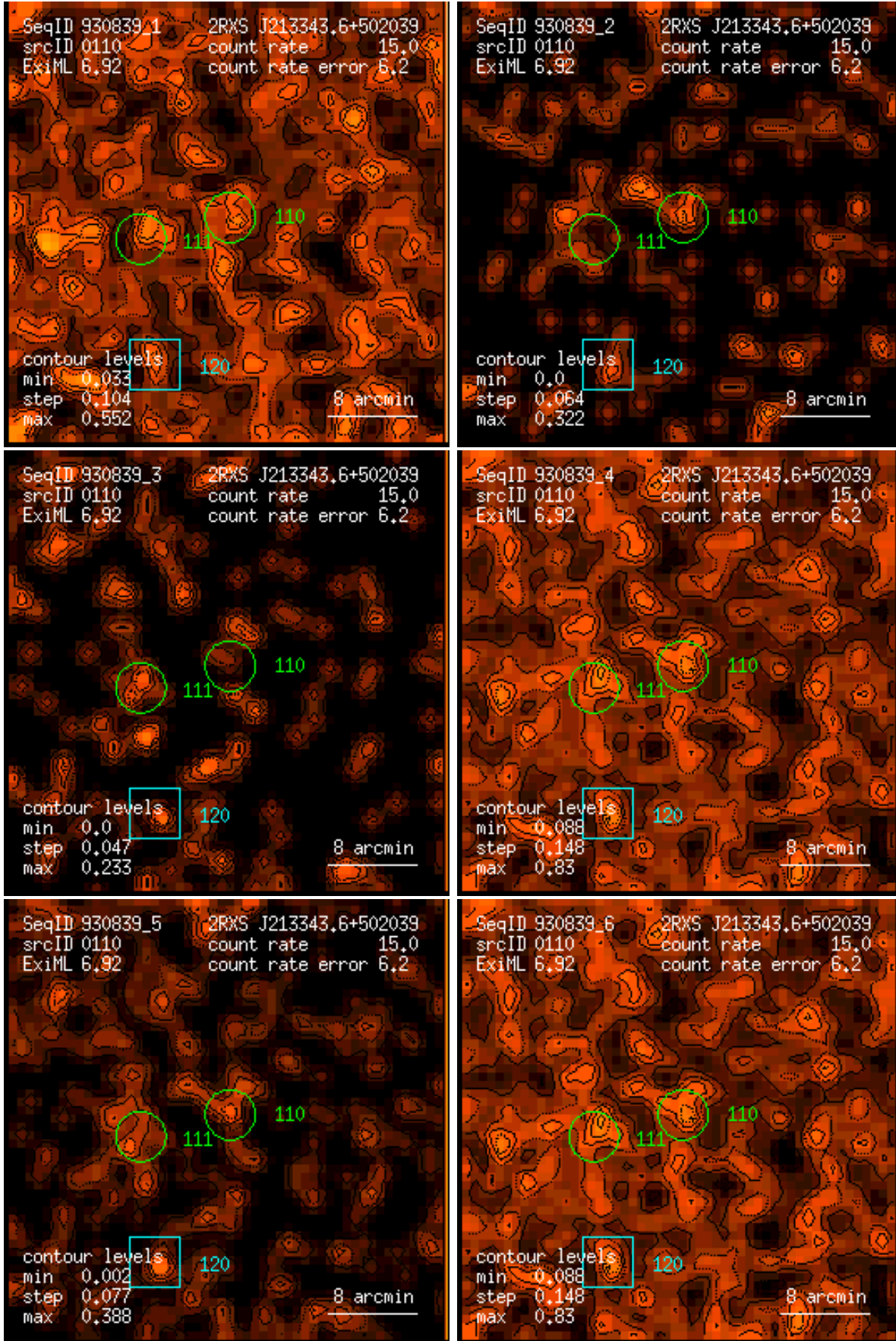
Figure 110: RASS 930839: detection 0110: band rate images, Gaussian filter: (1) PSPC channels 11 – 41, (2) 52 – 90, (3) 91 – 201, (4) 11 – 235, (5) 52 – 201, (6) 11 – 201. Broad band rates in counts/ks. Band rate contour levels in counts/ks/arcmin 2 .
