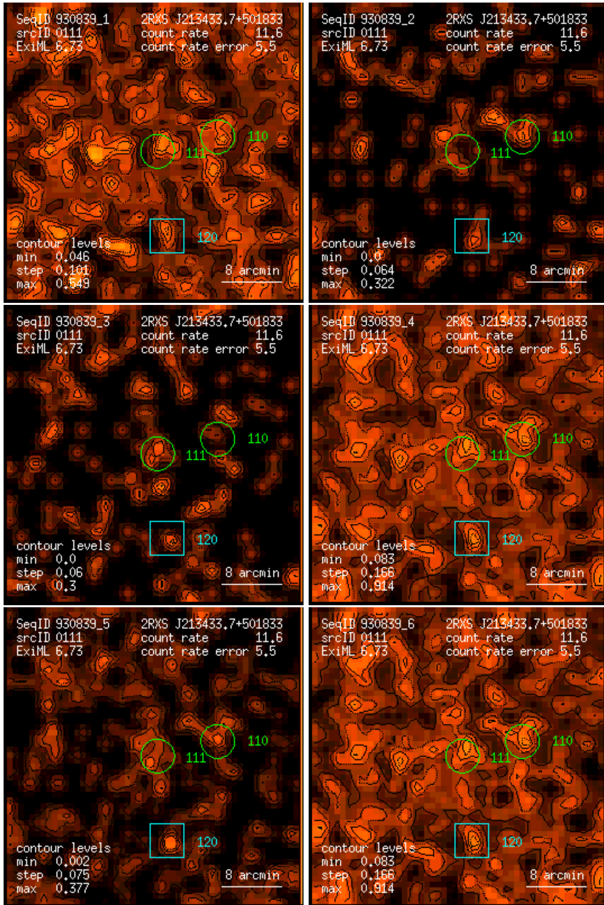
Figure 111: RASS 930839: detection 0111: band rate images, Gaussian filter: (1) PSPC channels 11 – 41, (2) 52 – 90, (3) 91 – 201, (4) 11 – 235, (5) 52 – 201, (6) 11 – 201. Broad band rates in counts/ks. Band rate contour levels in counts/ks/arcmin 2 .
