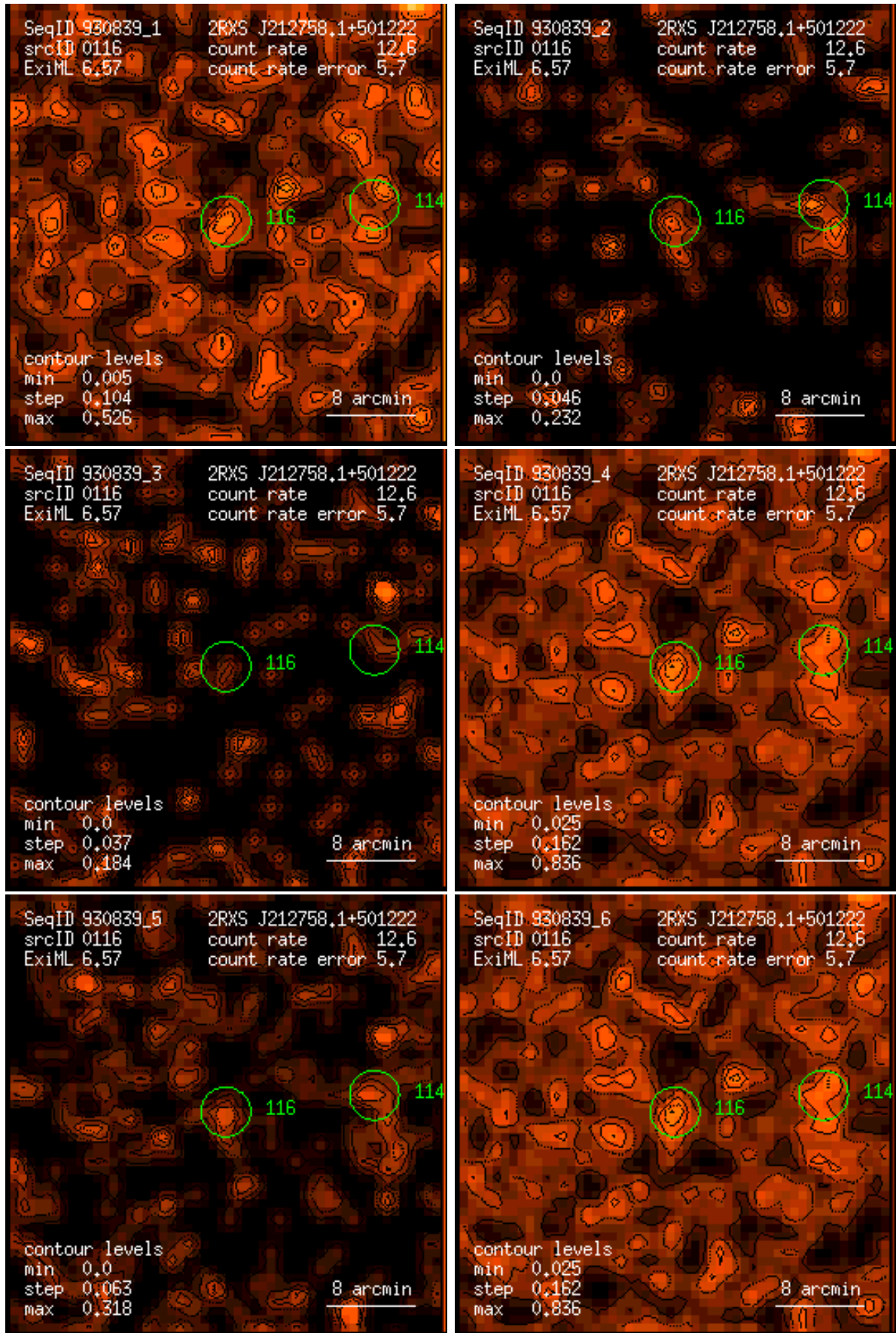
Figure 116: RASS 930839: detection 0116: band rate images, Gaussian filter: (1) PSPC channels 11 – 41, (2) 52 – 90, (3) 91 – 201, (4) 11 – 235, (5) 52 – 201, (6) 11 – 201. Broad band rates in counts/ks. Band rate contour levels in counts/ks/arcmin 2 .
