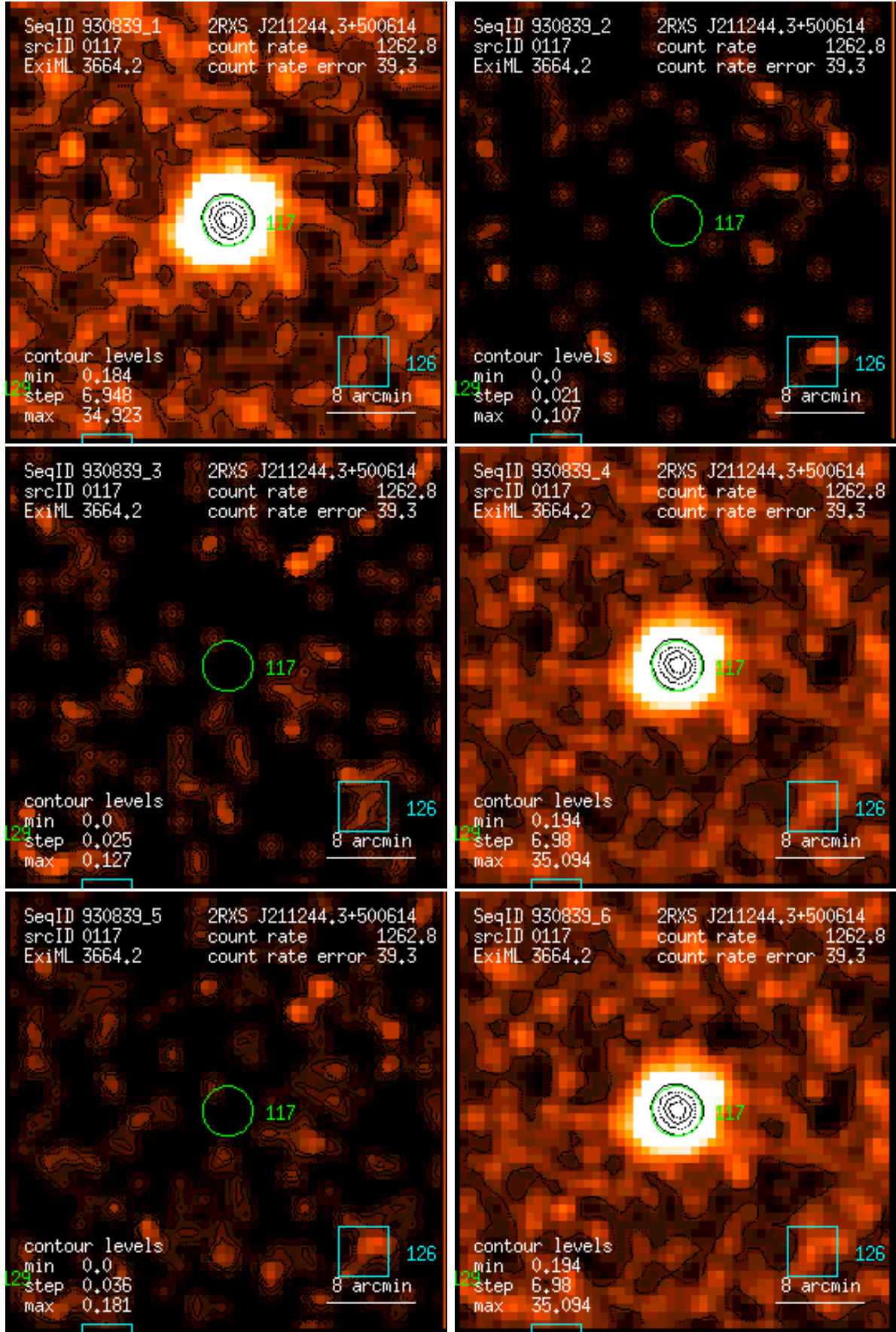
Figure 117: RASS 930839: detection 0117: band rate images, Gaussian filter: (1) PSPC channels 11 – 41, (2) 52 – 90, (3) 91 – 201, (4) 11 – 235, (5) 52 – 201, (6) 11 – 201. Broad band rates in counts/ks. Band rate contour levels in counts/ks/arcmin 2 .
