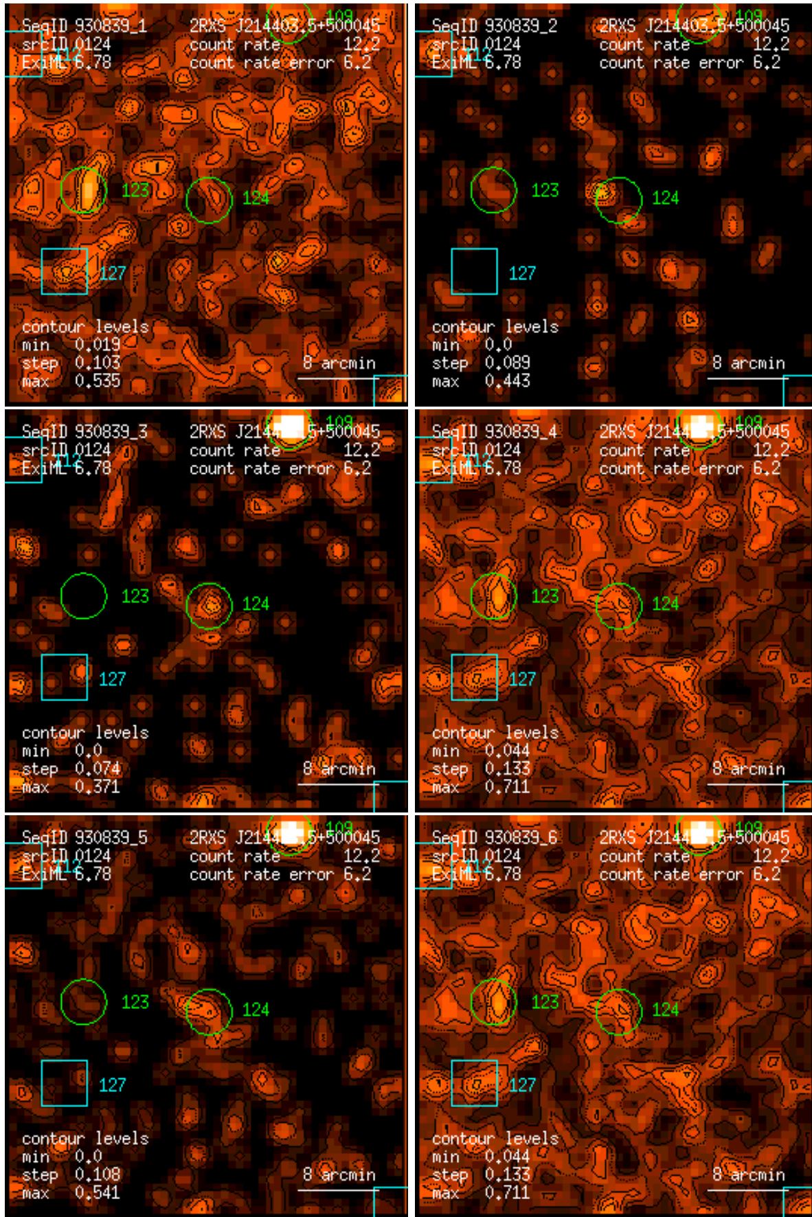
Figure 124: RASS 930839: detection 0124: band rate images, Gaussian filter: (1) PSPC channels 11 – 41, (2) 52 – 90, (3) 91 – 201, (4) 11 – 235, (5) 52 – 201, (6) 11 – 201. Broad band rates in counts/ks. Band rate contour levels in counts/ks/arcmin 2 .
