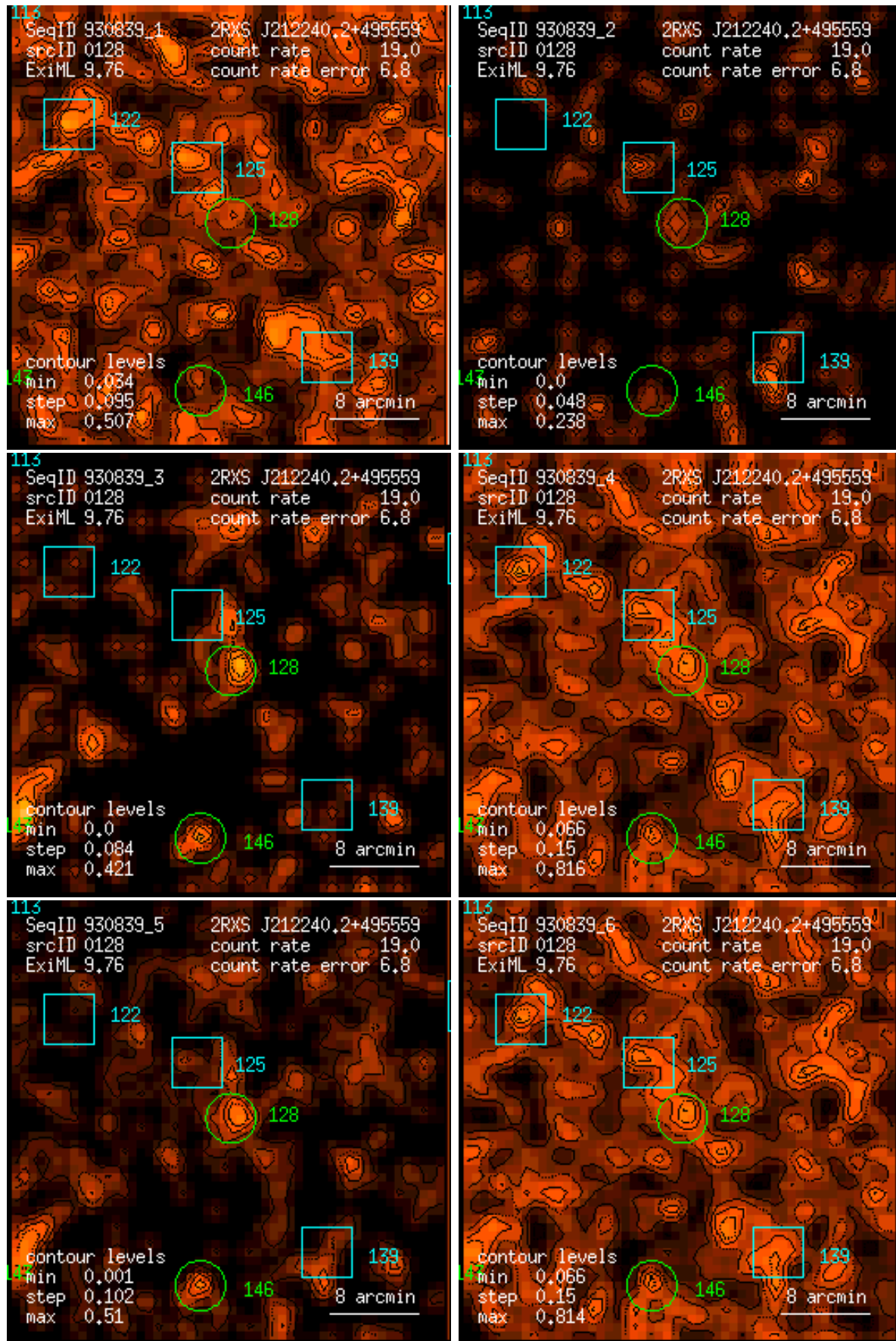
Figure 128: RASS 930839: detection 0128: band rate images, Gaussian filter: (1) PSPC channels 11 – 41, (2) 52 – 90, (3) 91 – 201, (4) 11 – 235, (5) 52 – 201, (6) 11 – 201. Broad band rates in counts/ks. Band rate contour levels in counts/ks/arcmin 2 .
