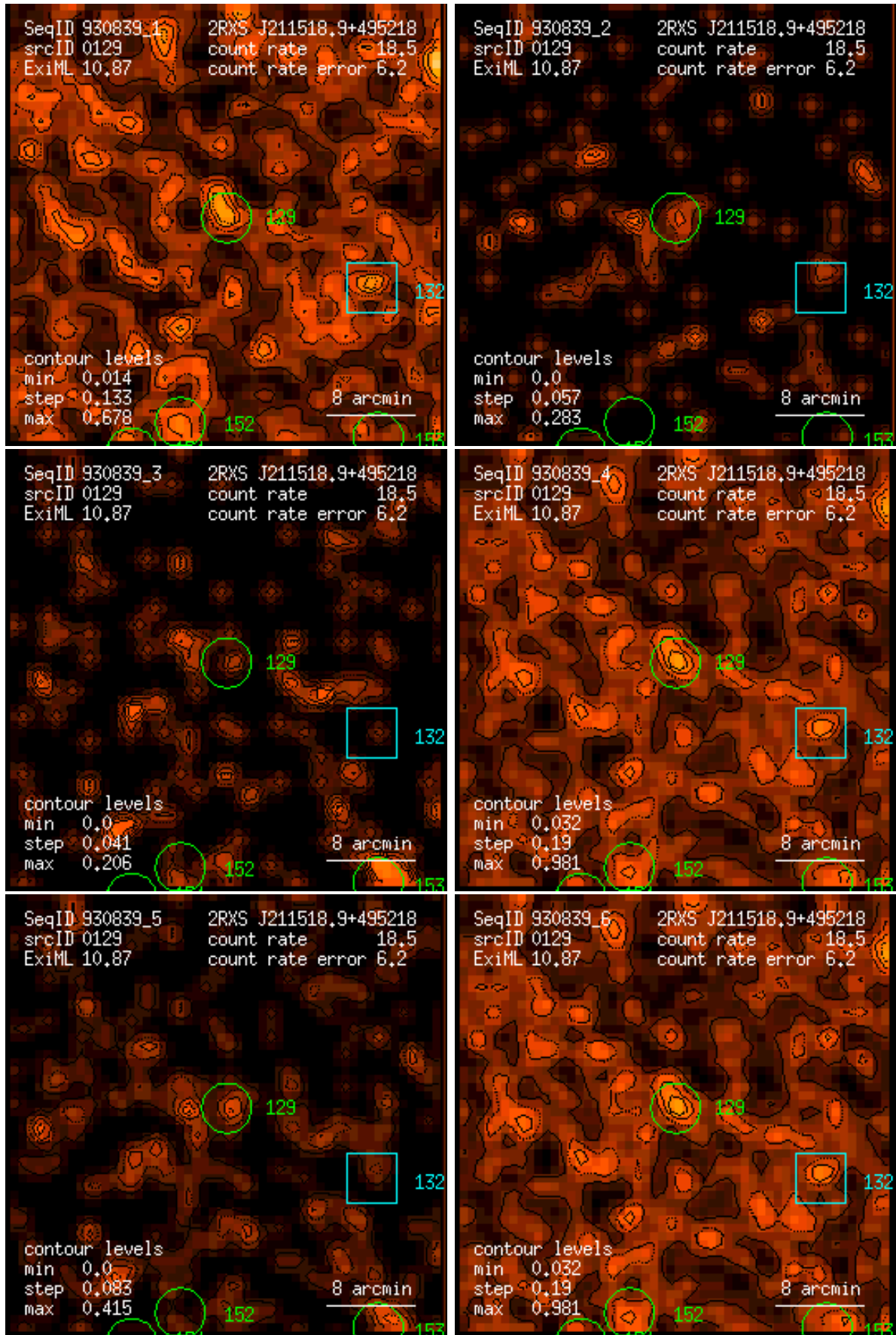
Figure 129: RASS 930839: detection 0129: band rate images, Gaussian filter: (1) PSPC channels 11 – 41, (2) 52 – 90, (3) 91 – 201, (4) 11 – 235, (5) 52 – 201, (6) 11 – 201. Broad band rates in counts/ks. Band rate contour levels in counts/ks/arcmin 2 .
