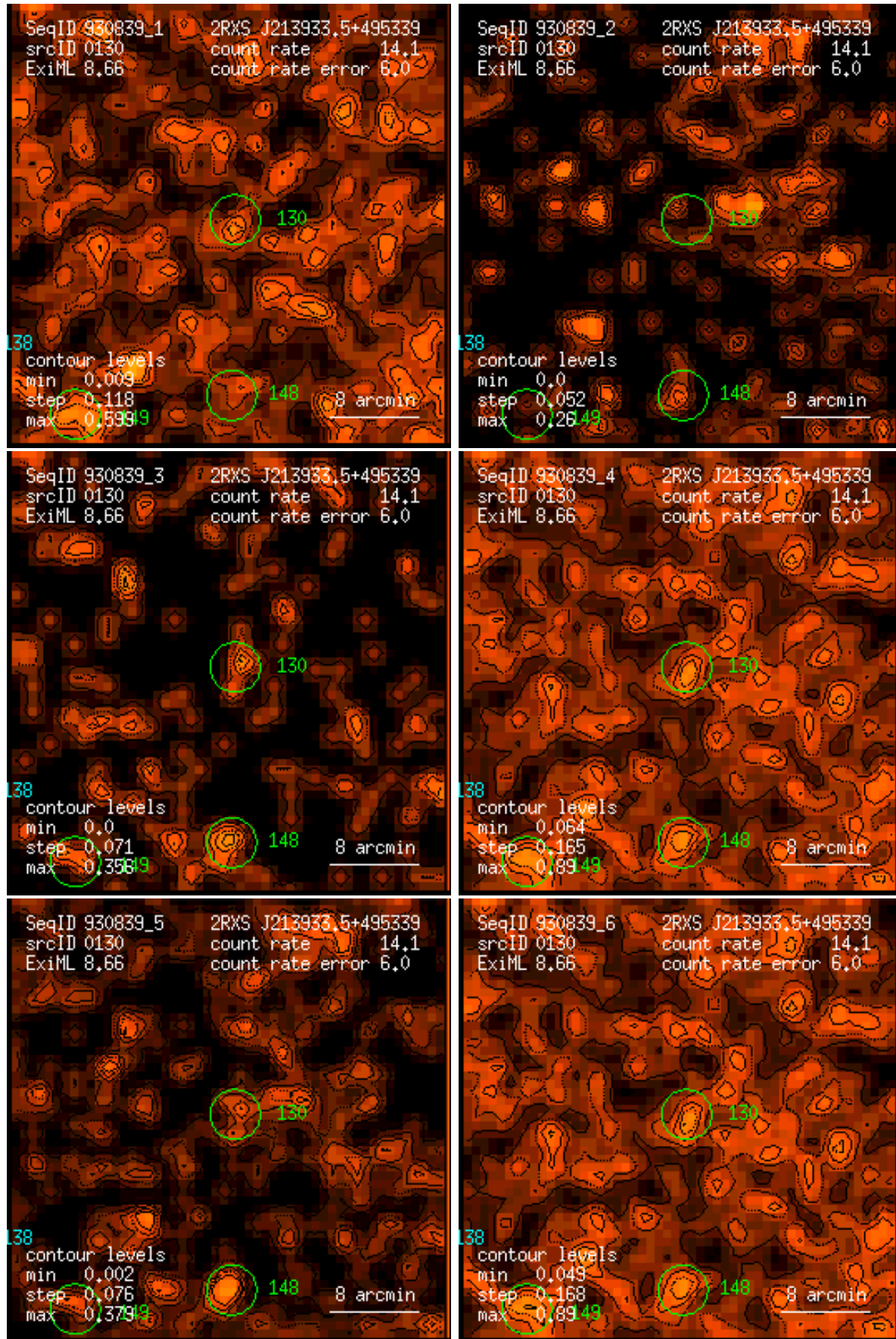
Figure 130: RASS 930839: detection 0130: band rate images, Gaussian filter: (1) PSPC channels 11 – 41, (2) 52 – 90, (3) 91 – 201, (4) 11 – 235, (5) 52 – 201, (6) 11 – 201. Broad band rates in counts/ks. Band rate contour levels in counts/ks/arcmin 2 .
