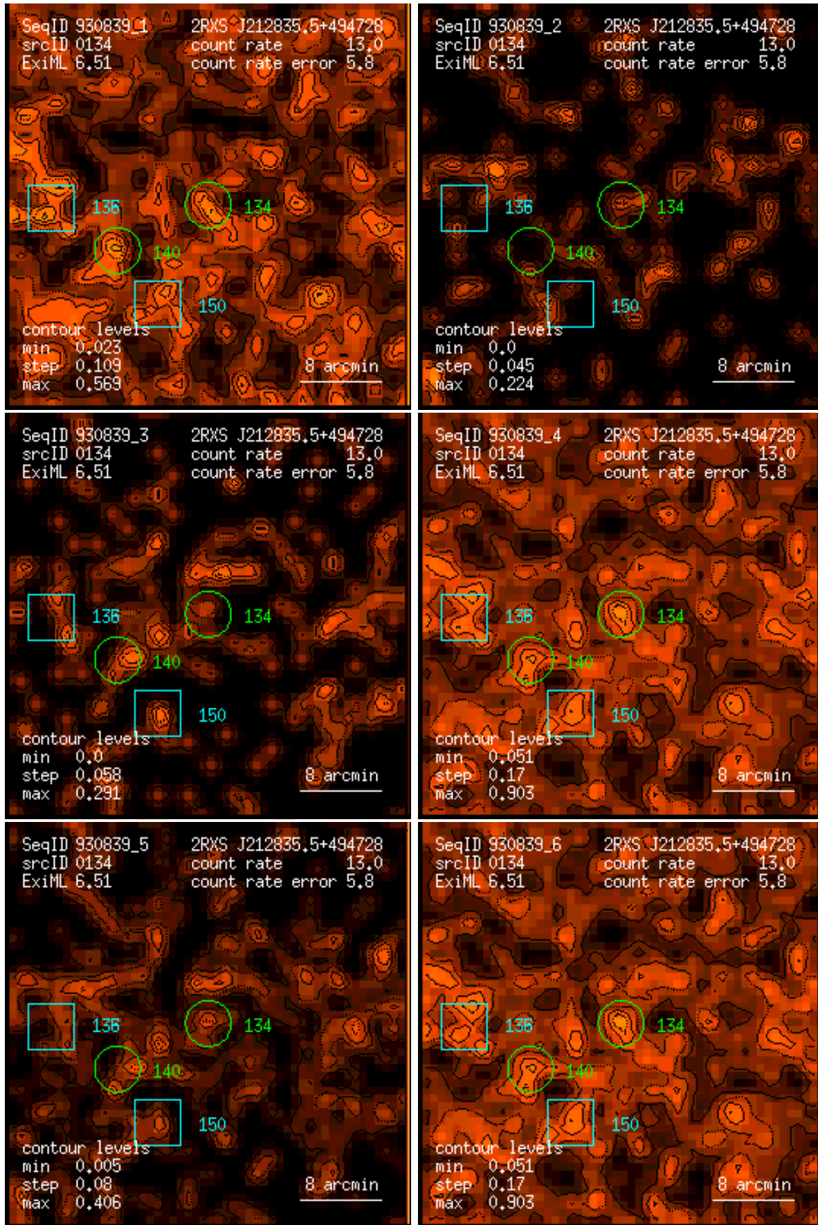
Figure 134: RASS 930839: detection 0134: band rate images, Gaussian filter: (1) PSPC channels 11 – 41, (2) 52 – 90, (3) 91 – 201, (4) 11 – 235, (5) 52 – 201, (6) 11 – 201. Broad band rates in counts/ks. Band rate contour levels in counts/ks/arcmin 2 .
