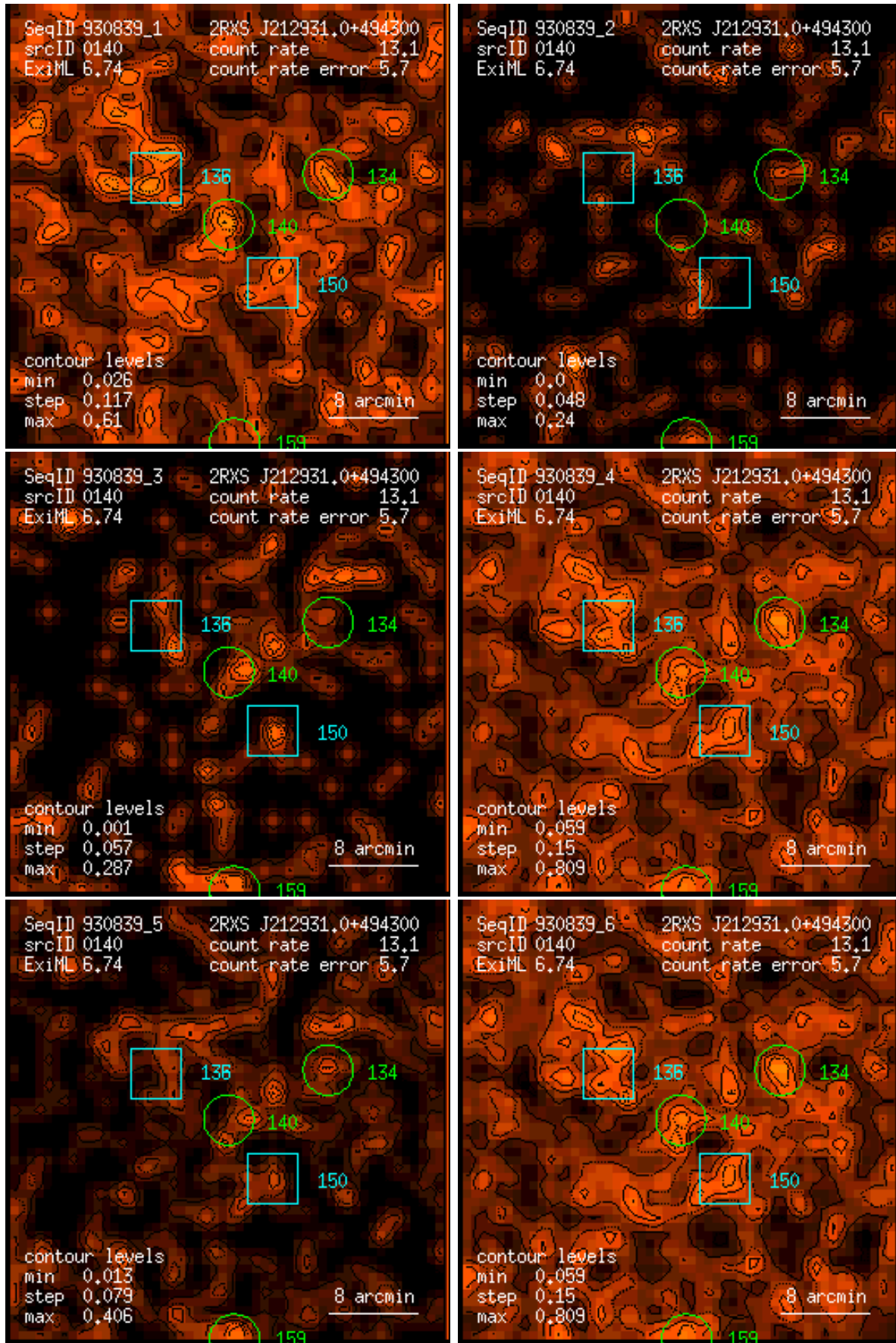
Figure 140: RASS 930839: detection 0140: band rate images, Gaussian filter: (1) PSPC channels 11 – 41, (2) 52 – 90, (3) 91 – 201, (4) 11 – 235, (5) 52 – 201, (6) 11 – 201. Broad band rates in counts/ks. Band rate contour levels in counts/ks/arcmin 2 .
