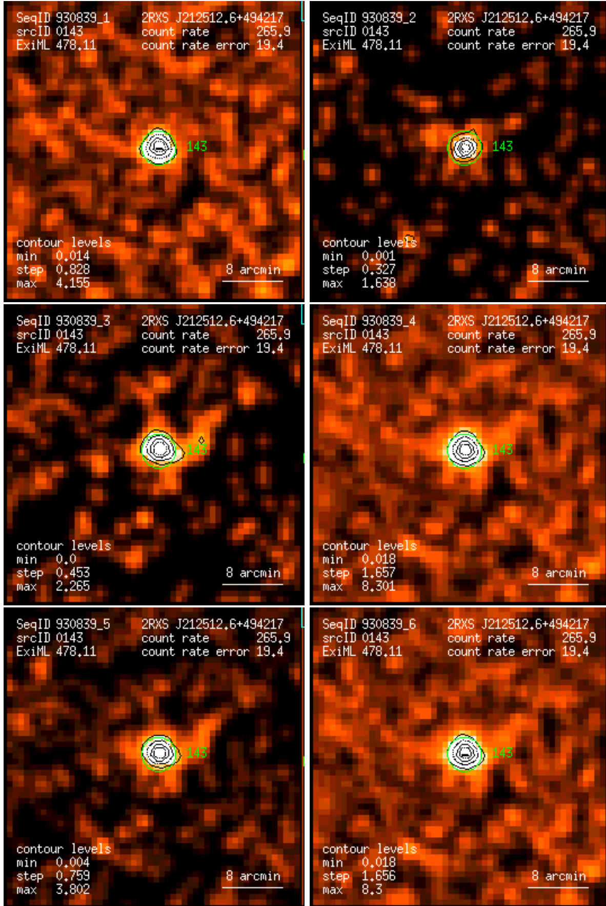
Figure 143: RASS 930839: detection 0143: band rate images, Gaussian filter: (1) PSPC channels 11 – 41, (2) 52 – 90, (3) 91 – 201, (4) 11 – 235, (5) 52 – 201, (6) 11 – 201. Broad band rates in counts/ks. Band rate contour levels in counts/ks/arcmin 2 .
