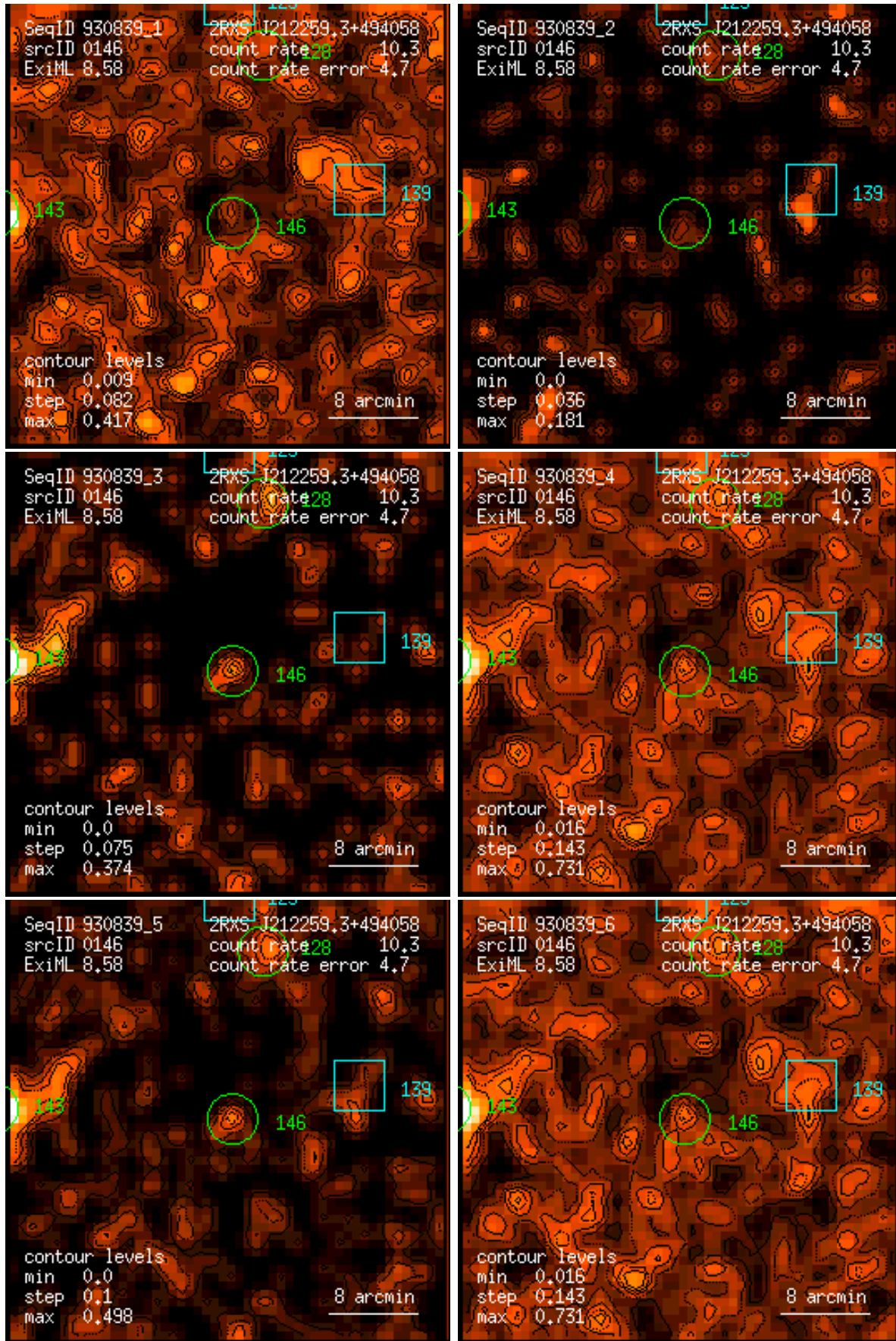
Figure 146: RASS 930839: detection 0146: band rate images, Gaussian filter: (1) PSPC channels 11 – 41, (2) 52 – 90, (3) 91 – 201, (4) 11 – 235, (5) 52 – 201, (6) 11 – 201. Broad band rates in counts/ks. Band rate contour levels in counts/ks/arcmin 2 .
