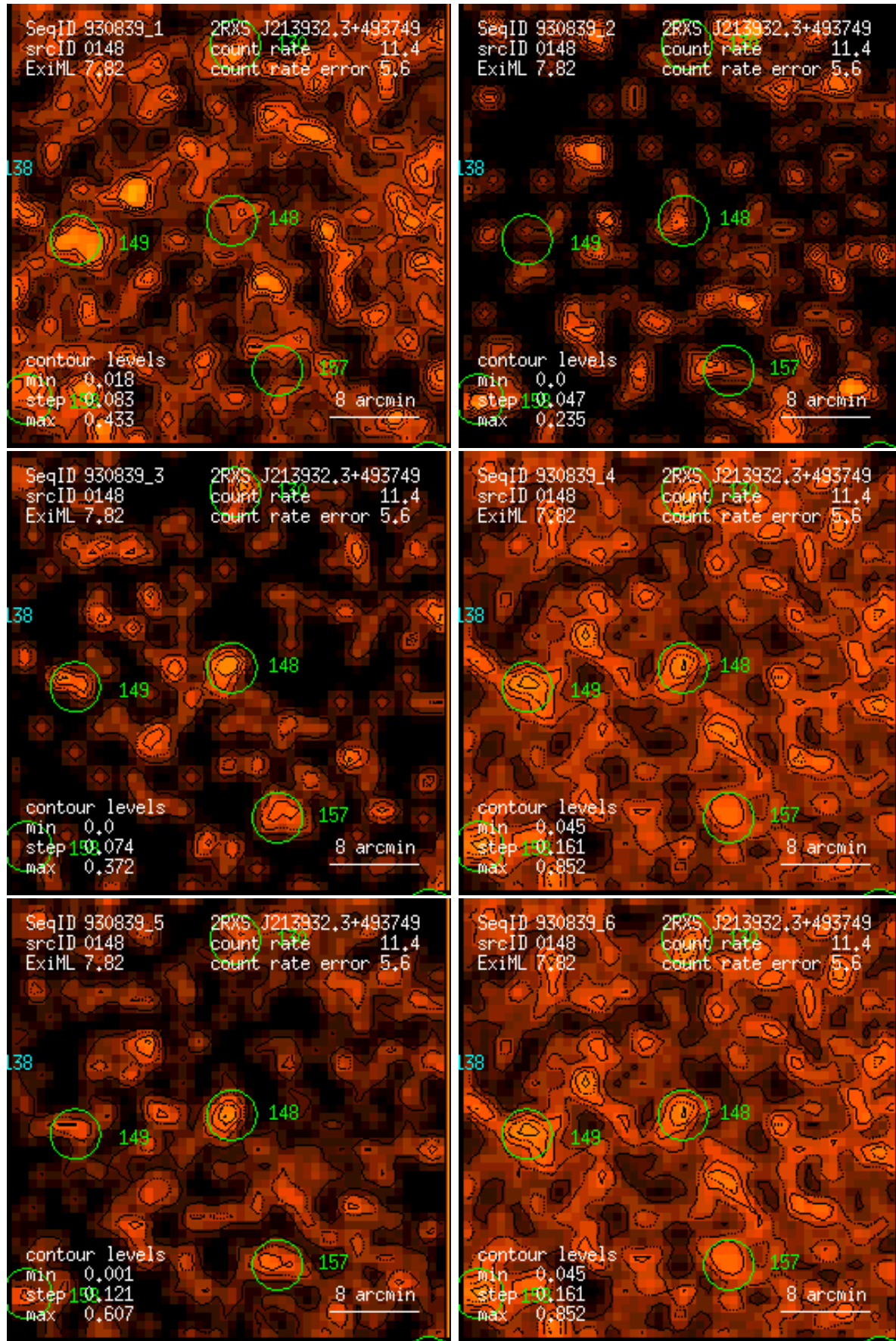
Figure 148: RASS 930839: detection 0148: band rate images, Gaussian filter: (1) PSPC channels 11 – 41, (2) 52 – 90, (3) 91 – 201, (4) 11 – 235, (5) 52 – 201, (6) 11 – 201. Broad band rates in counts/ks. Band rate contour levels in counts/ks/arcmin 2 .
