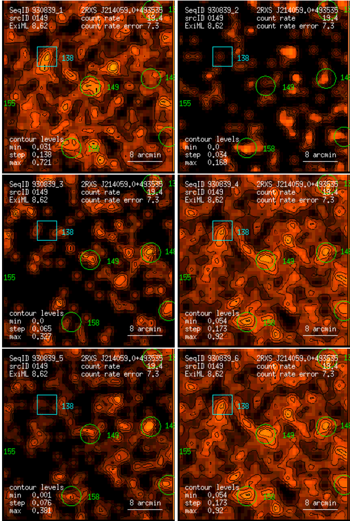
Figure 149: RASS 930839: detection 0149: band rate images, Gaussian filter: (1) PSPC channels 11 – 41, (2) 52 – 90, (3) 91 – 201, (4) 11 – 235, (5) 52 – 201, (6) 11 – 201. Broad band rates in counts/ks. Band rate contour levels in counts/ks/arcmin 2 .
