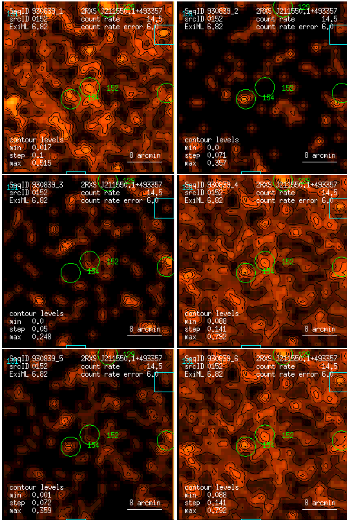
Figure 152: RASS 930839: detection 0152: band rate images, Gaussian filter: (1) PSPC channels 11 – 41, (2) 52 – 90, (3) 91 – 201, (4) 11 – 235, (5) 52 – 201, (6) 11 – 201. Broad band rates in counts/ks. Band rate contour levels in counts/ks/arcmin 2 .
