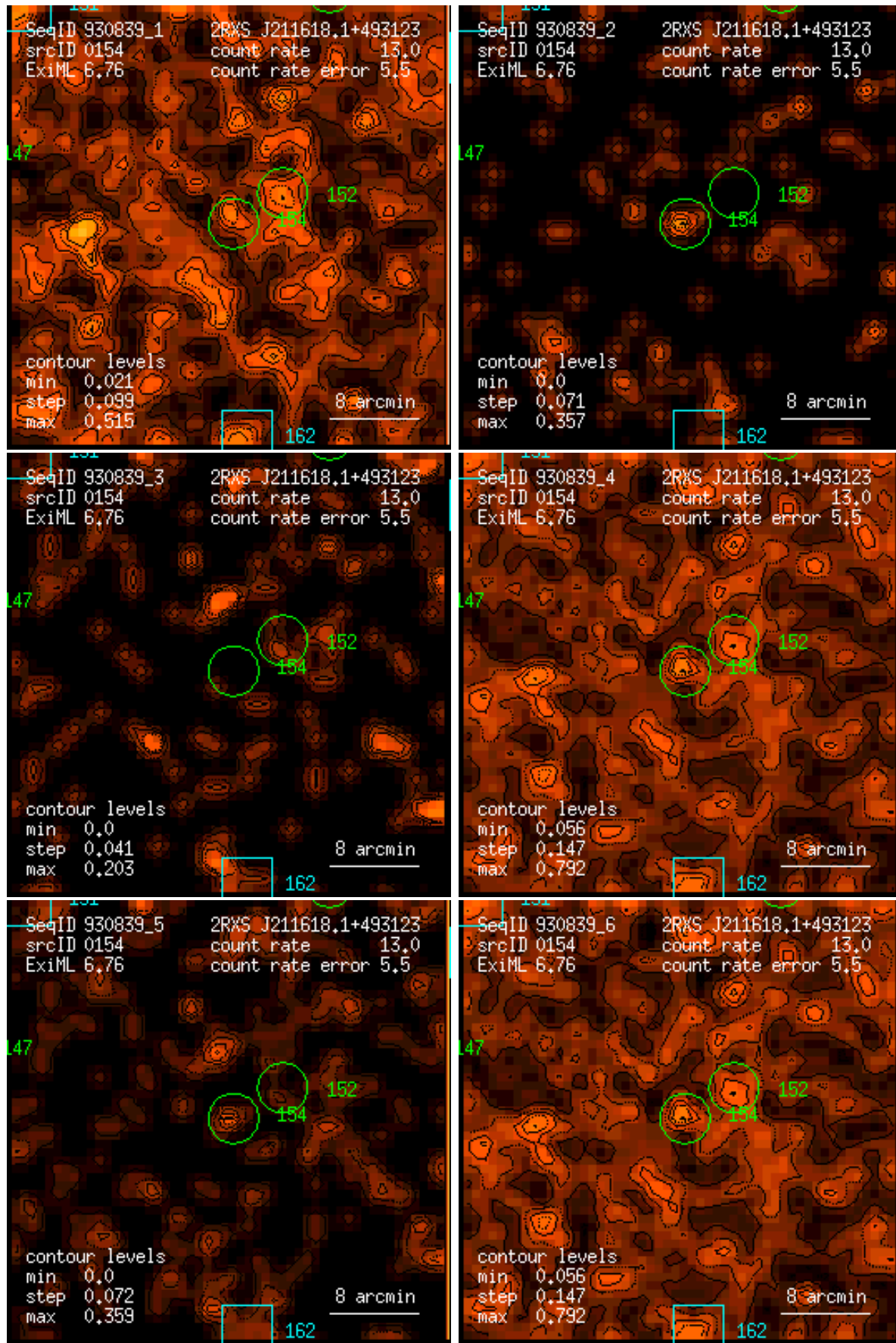
Figure 154: RASS 930839: detection 0154: band rate images, Gaussian filter: (1) PSPC channels 11 – 41, (2) 52 – 90, (3) 91 – 201, (4) 11 – 235, (5) 52 – 201, (6) 11 – 201. Broad band rates in counts/ks. Band rate contour levels in counts/ks/arcmin 2 .
