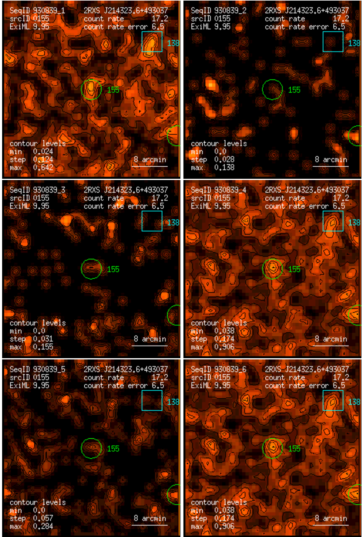
Figure 155: RASS 930839: detection 0155: band rate images, Gaussian filter: (1) PSPC channels 11 – 41, (2) 52 – 90, (3) 91 – 201, (4) 11 – 235, (5) 52 – 201, (6) 11 – 201. Broad band rates in counts/ks. Band rate contour levels in counts/ks/arcmin 2 .
