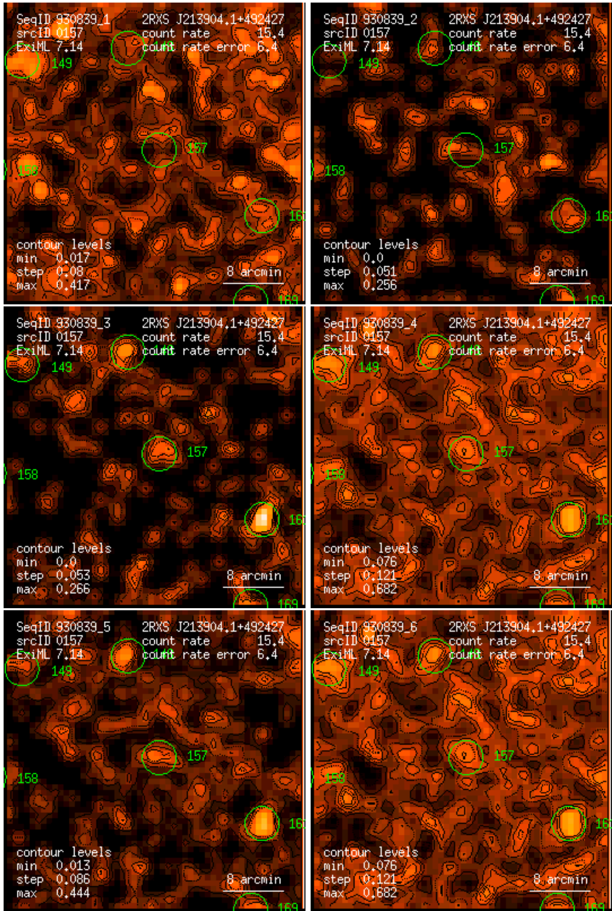
Figure 157: RASS 930839: detection 0157: band rate images, Gaussian filter: (1) PSPC channels 11 – 41, (2) 52 – 90, (3) 91 – 201, (4) 11 – 235, (5) 52 – 201, (6) 11 – 201. Broad band rates in counts/ks. Band rate contour levels in counts/ks/arcmin 2 .
