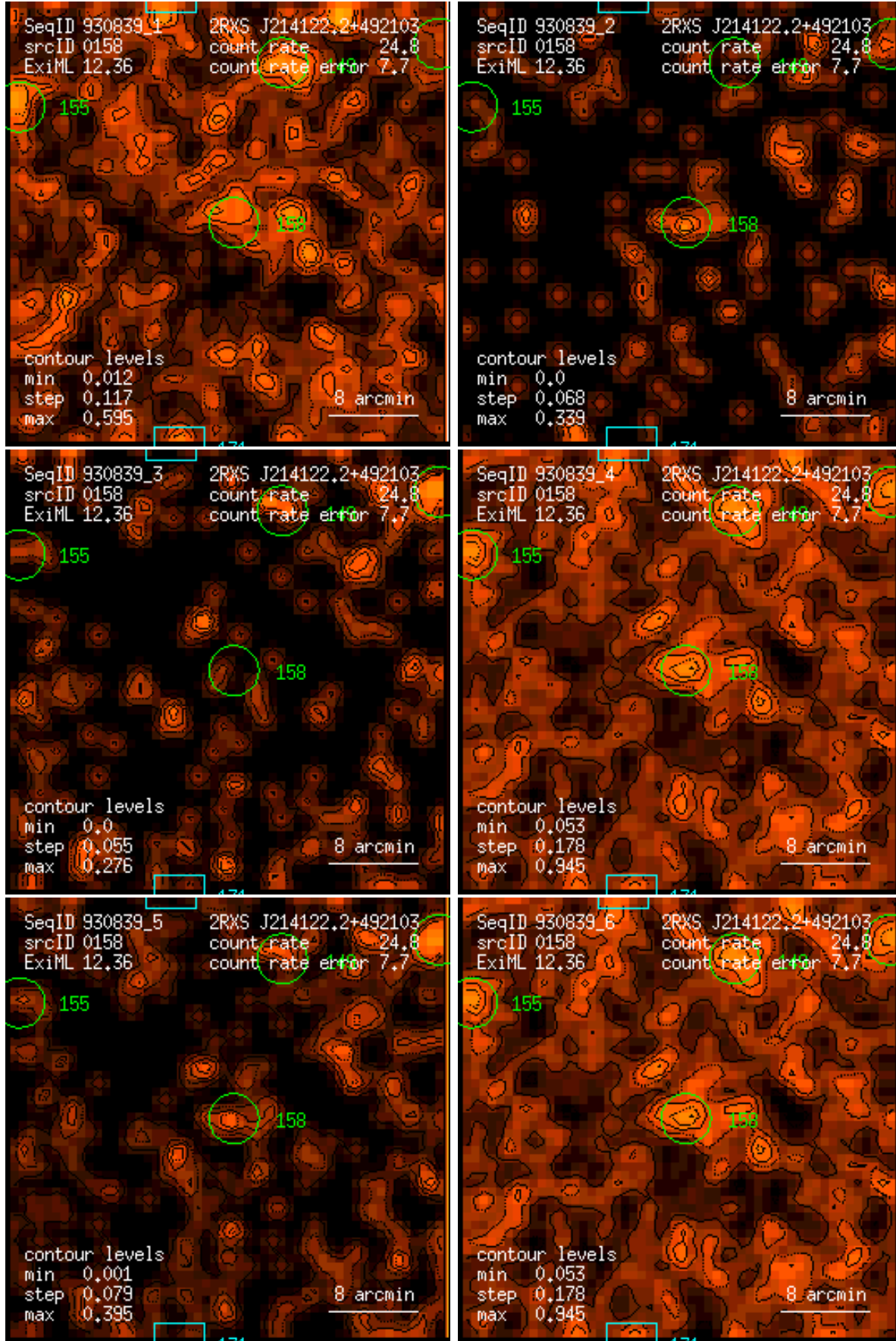
Figure 158: RASS 930839: detection 0158: band rate images, Gaussian filter: (1) PSPC channels 11 – 41, (2) 52 – 90, (3) 91 – 201, (4) 11 – 235, (5) 52 – 201, (6) 11 – 201. Broad band rates in counts/ks. Band rate contour levels in counts/ks/arcmin 2 .
