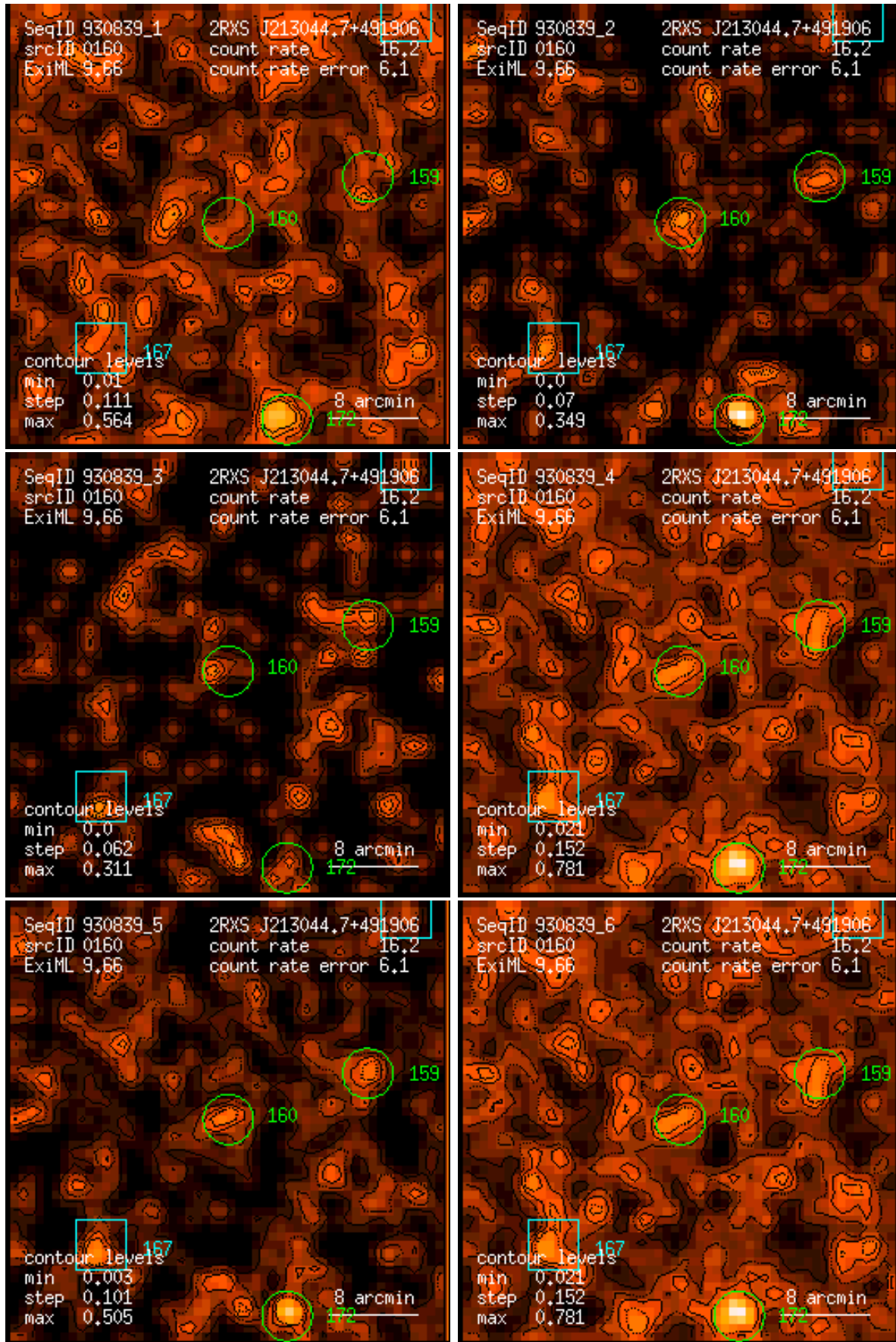
Figure 160: RASS 930839: detection 0160: band rate images, Gaussian filter: (1) PSPC channels 11 – 41, (2) 52 – 90, (3) 91 – 201, (4) 11 – 235, (5) 52 – 201, (6) 11 – 201. Broad band rates in counts/ks. Band rate contour levels in counts/ks/arcmin 2 .
