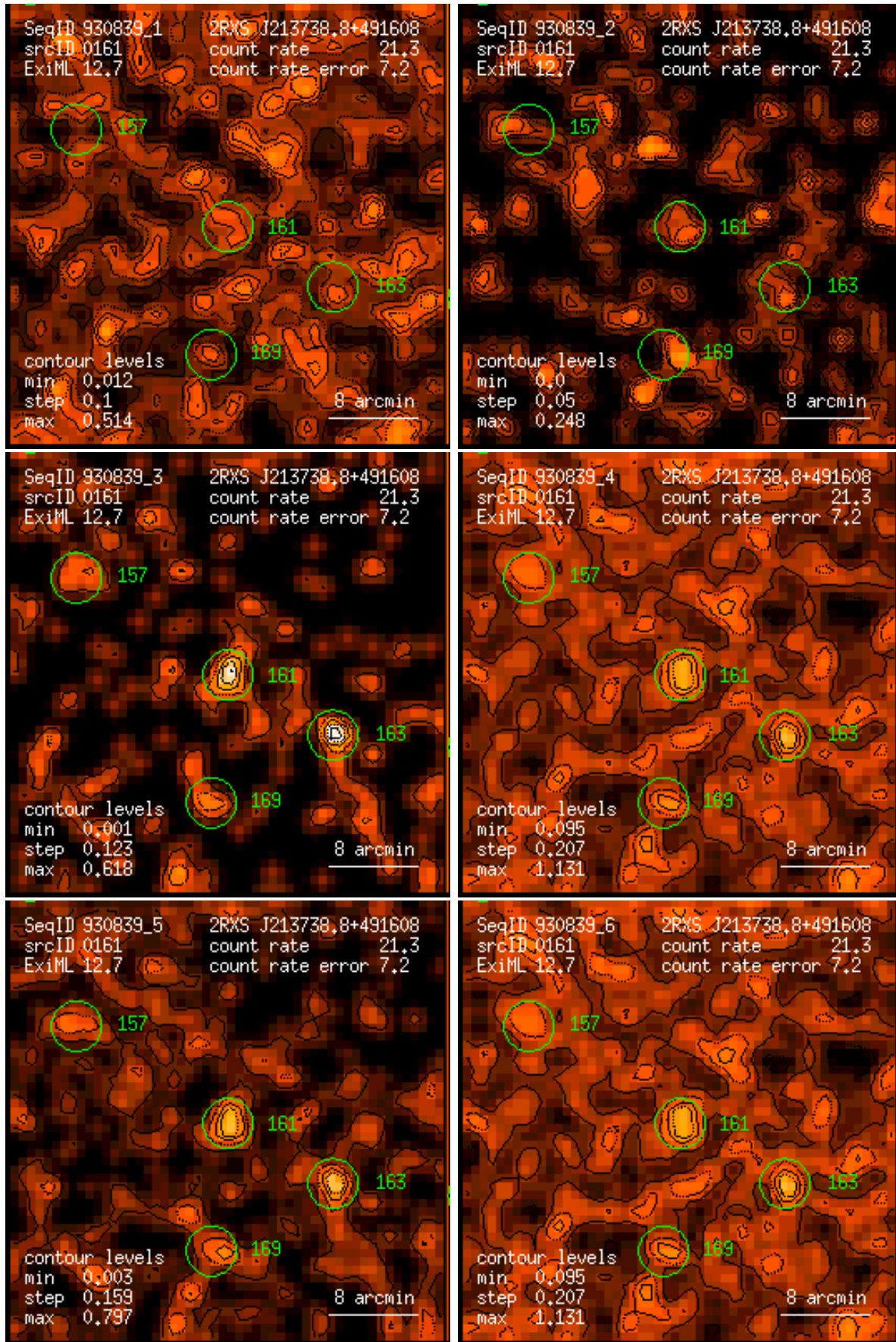
Figure 161: RASS 930839: detection 0161: band rate images, Gaussian filter: (1) PSPC channels 11 – 41, (2) 52 – 90, (3) 91 – 201, (4) 11 – 235, (5) 52 – 201, (6) 11 – 201. Broad band rates in counts/ks. Band rate contour levels in counts/ks/arcmin 2 .
